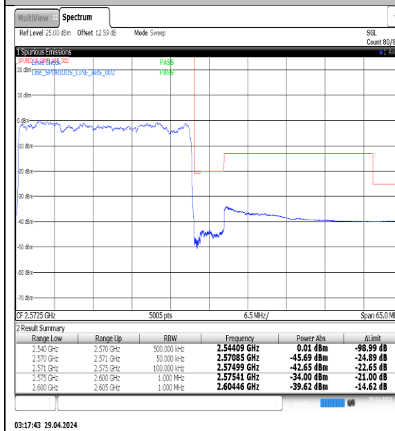
NTNV-N7-PC3-15-30-H-DFT-QPSK-Outer_Full-Ant1-PASS
