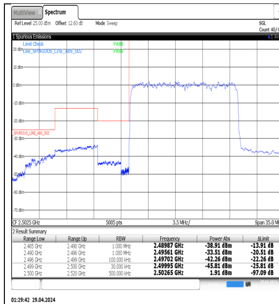
NTNV-N7-PC3-15-15-L-DFT-QPSK-Outer_Full- Ant1-PASS
