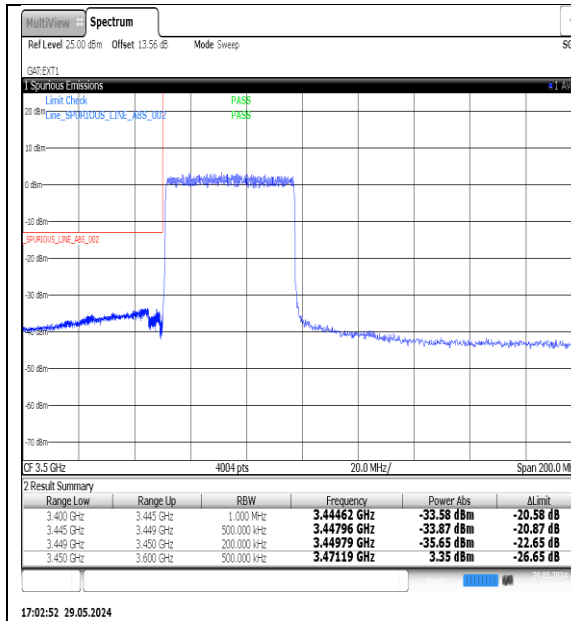
NTNV-N77-3450-3550-PC3-30-50-L-DFT-QPSK- Outer_Full-Ant1-PASS
