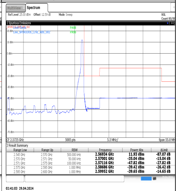
NTNV-N7-PC3-15-25-H-DFT-QPSK-Edge_1RB_Right-Ant1-PASS
