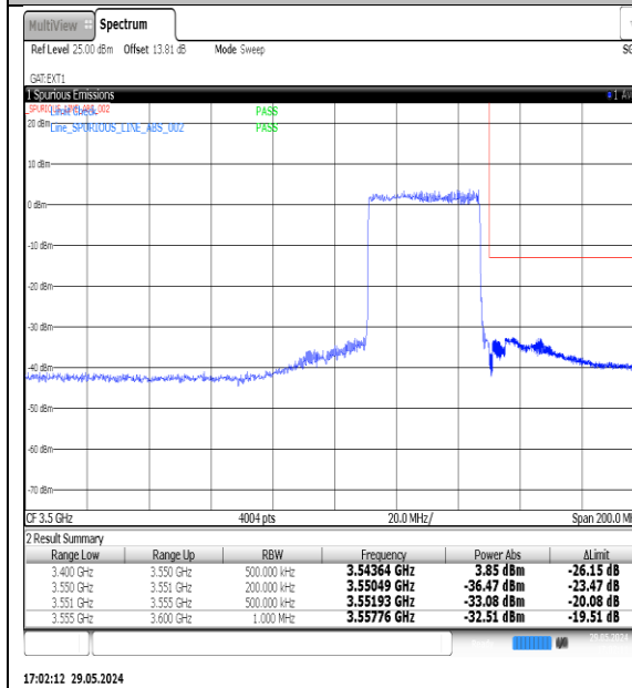
NTNV-N77-3450-3550-PC3-30-40-H-DFT-QPSK- Outer_Full-Ant1-PASS
