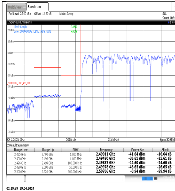
NTNV-N7-PC3-15-25-L-DFT-QPSK-Outer_Full-Ant1-PASS
