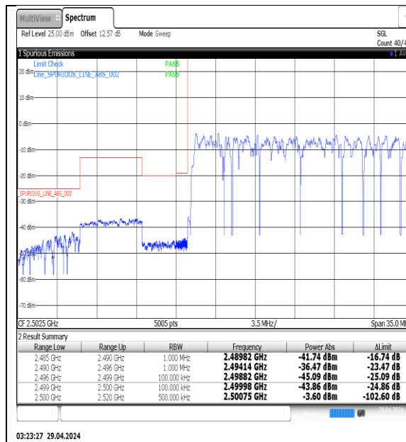
NTNV-N7-PC3-15-40-L-DFT-QPSK-Outer_Full- Ant1-PASS
