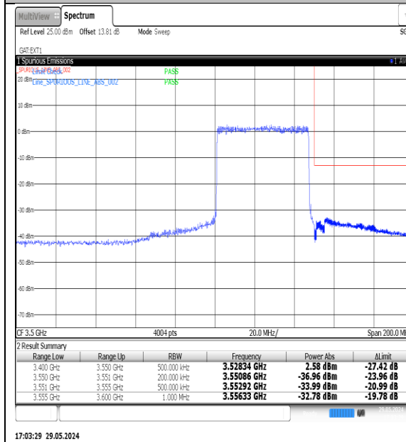
NTNV-N77-3450-3550-PC3-30-50-H-DFT-QPSK- Outer_Full-Ant1-PASS
