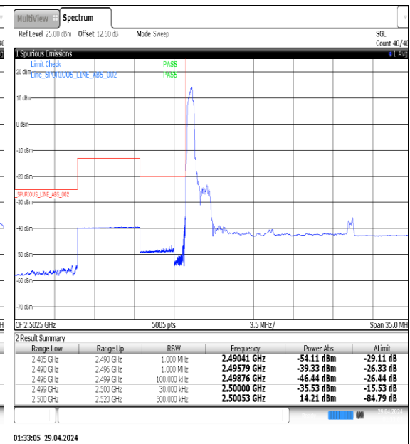
NTNV-N7-PC3-15-15-L-DFT-QPSK- Edge_1RB_Left-Ant1-PASS
