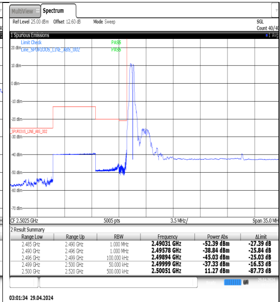
NTNV-N7-PC3-15-30-L-DFT-QPSK-Edge_1RB_Left-Ant1-PASS
