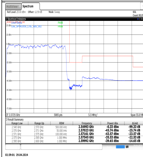
NTNV-N7-PC3-15-25-H-DFT-QPSK-Outer_Full-Ant1-PASS
