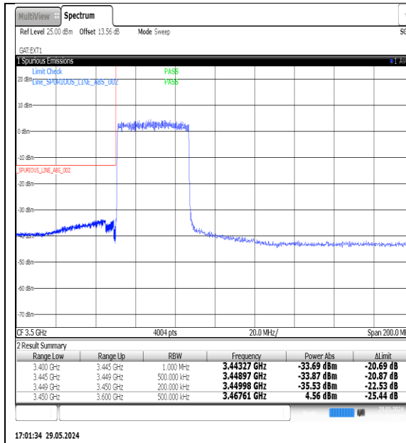
NTNV-N77-3450-3550-PC3-30-40-L-DFT-QPSK- Outer_Full-Ant1-PASS
