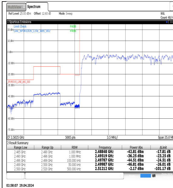
NTNV-N7-PC3-15-30-L-DFT-QPSK-Outer_Full-Ant1-PASS
