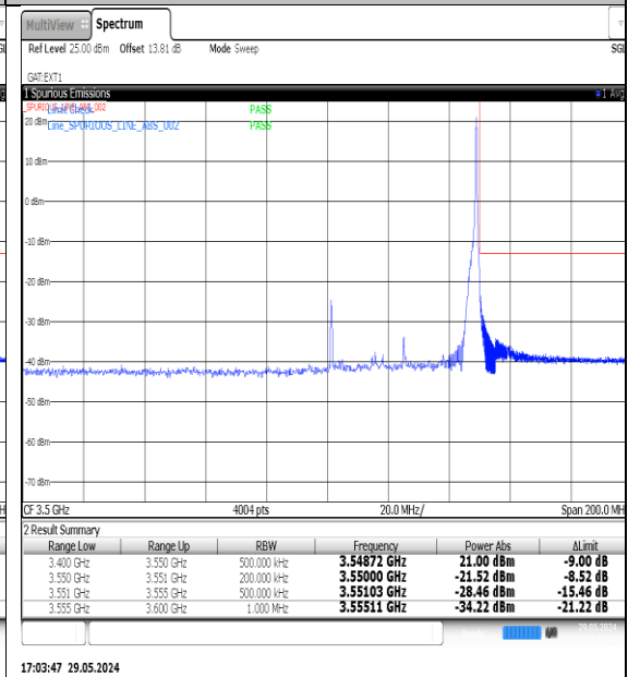
NTNV-N77-3450-3550-PC3-30-50-H-DFT-QPSK- Edge_1RB_Right-Ant1-PASS
