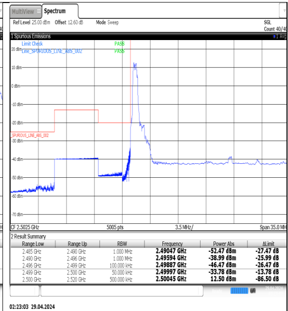
NTNV-N7-PC3-15-25-L-DFT-QPSK-Edge_1RB_Left-Ant1-PASS
