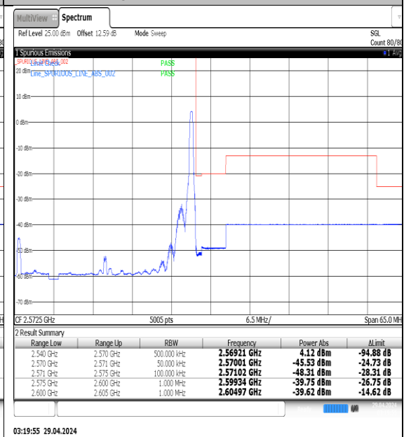
NTNV-N7-PC3-15-30-H-DFT-QPSK-Edge_1RB_Right-Ant1-PASS
