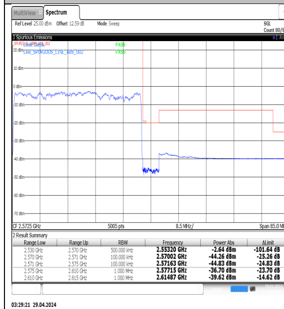
NTNV-N7-PC3-15-40-H-DFT-QPSK-Outer_Full- Ant1-PASS
