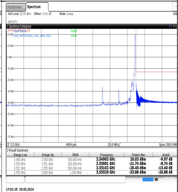
NTNV-N77-3450-3550-PC3-30-40-H-DFT-QPSK- Edge_1RB_Right-Ant1-PASS
