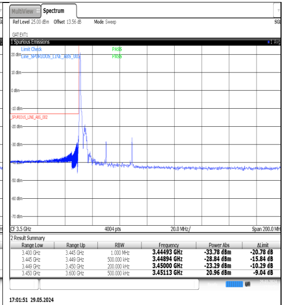
NTNV-N77-3450-3550-PC3-30-40-L-DFT-QPSK- Edge_1RB_Left-Ant1-PASS
