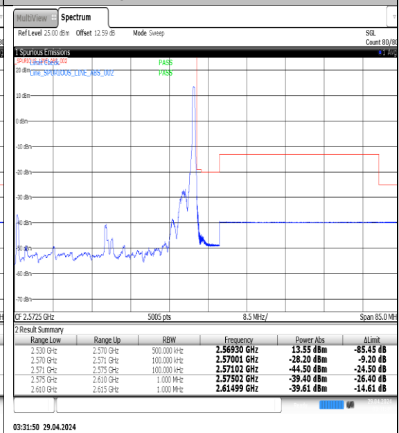
NTNV-N7-PC3-15-40-H-DFT-QPSK- Edge_1RB_Right-Ant1-PASS
