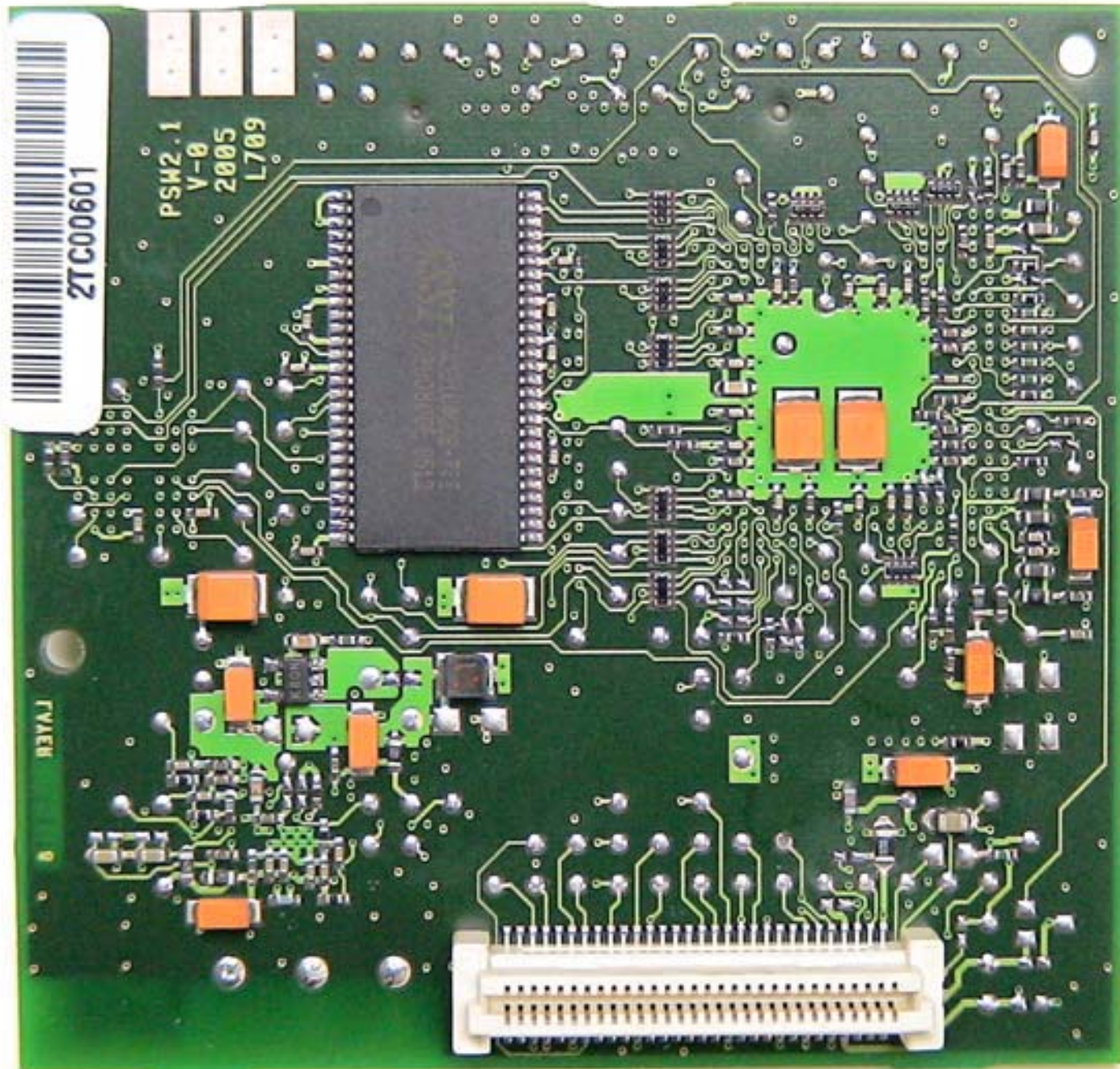
Bluetooth PCB (bottom)
