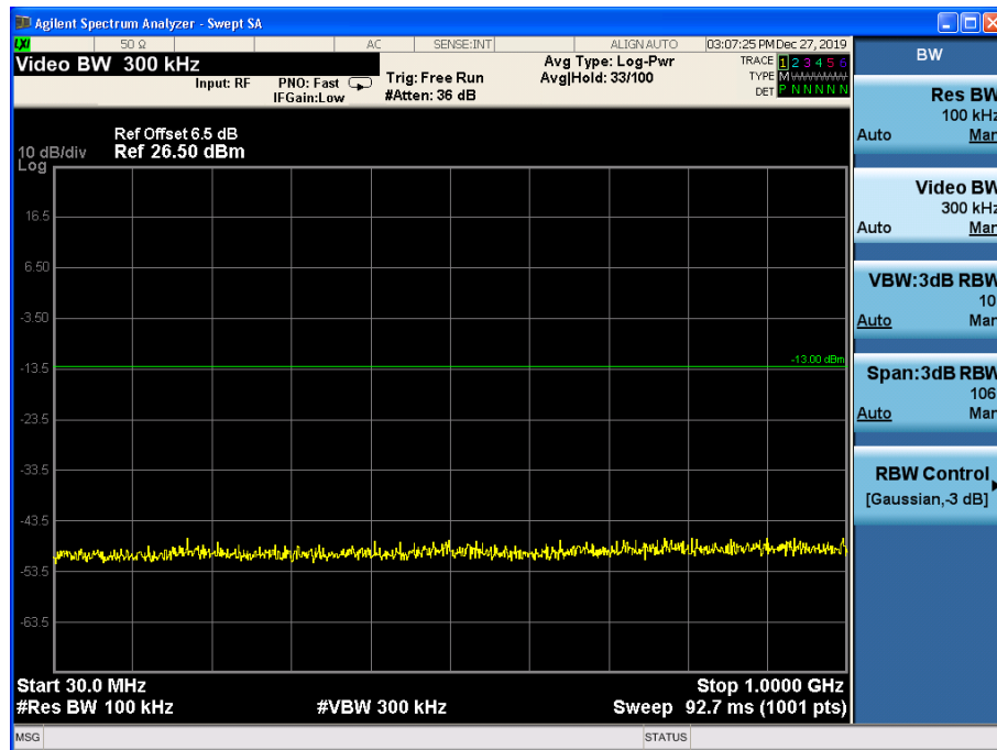
Channel 1412, 30MHz~1GHz
