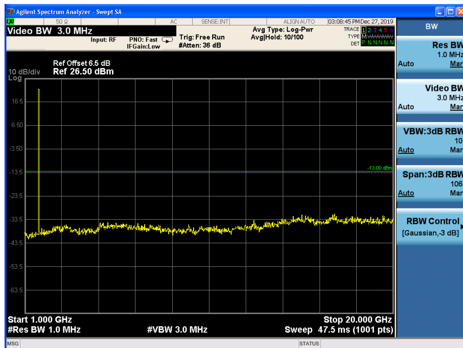
Channel 1412, 1GHz~20GHz
