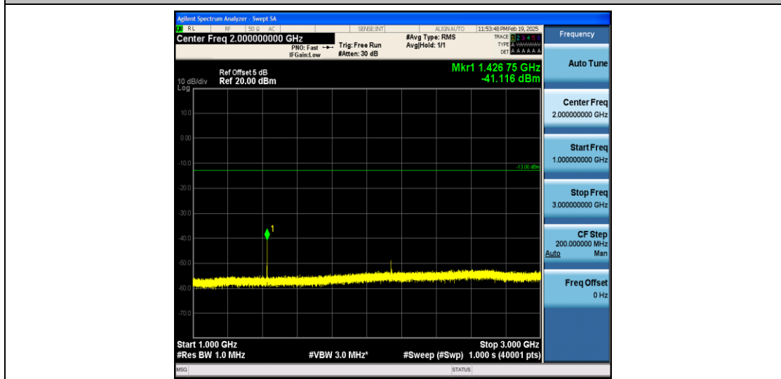
Band12_3MHz_16QAM_23165_1RB#0_1000~3000_1000~3000
