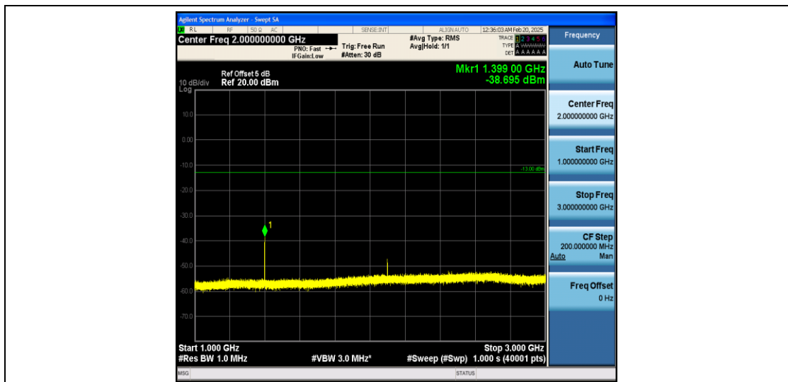
Band12_10MHz_QPSK_23060_1RB#0_1000~3000_1000~3000
