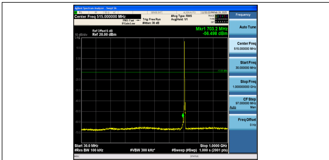
Band12_3MHz_16QAM_23165_1RB#0_30~1000_30~1000
