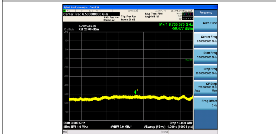
Band12_5MHz_QPSK_23035_1RB#0_3000~10000_3000~10000
