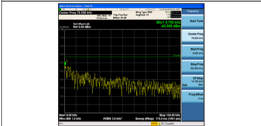
Band12_10MHz_16QAM_23060_1RB#0_0.009~0.15_0.009~0.15
