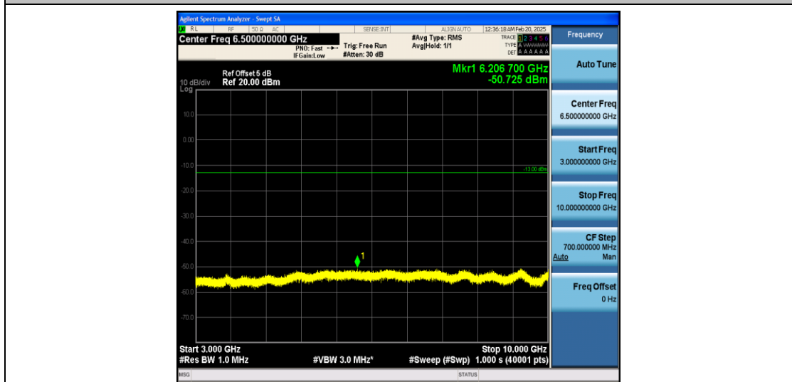
Band12_10MHz_QPSK_23060_1RB#0_3000~10000_3000~10000
