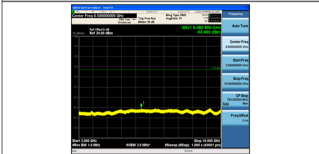
Band12_3MHz_16QAM_23095_1RB#0_3000~10000_3000~10000
