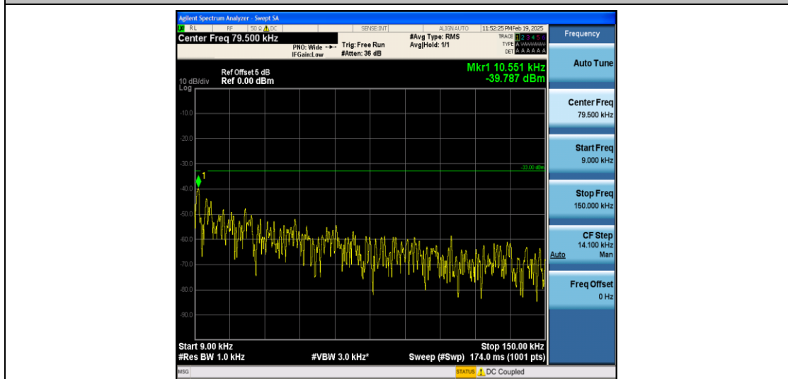
Band12_3MHz_QPSK_23165_1RB#0_0.009~0.15_0.009~0.15
