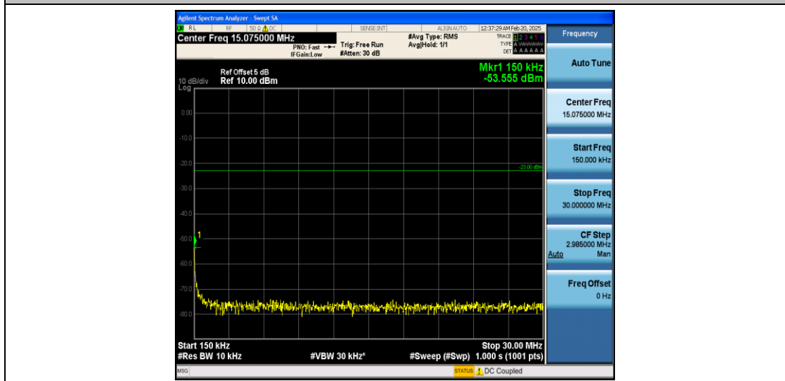
Band12_10MHz_QPSK_23095_1RB#0_0.15~30_0.15~30
