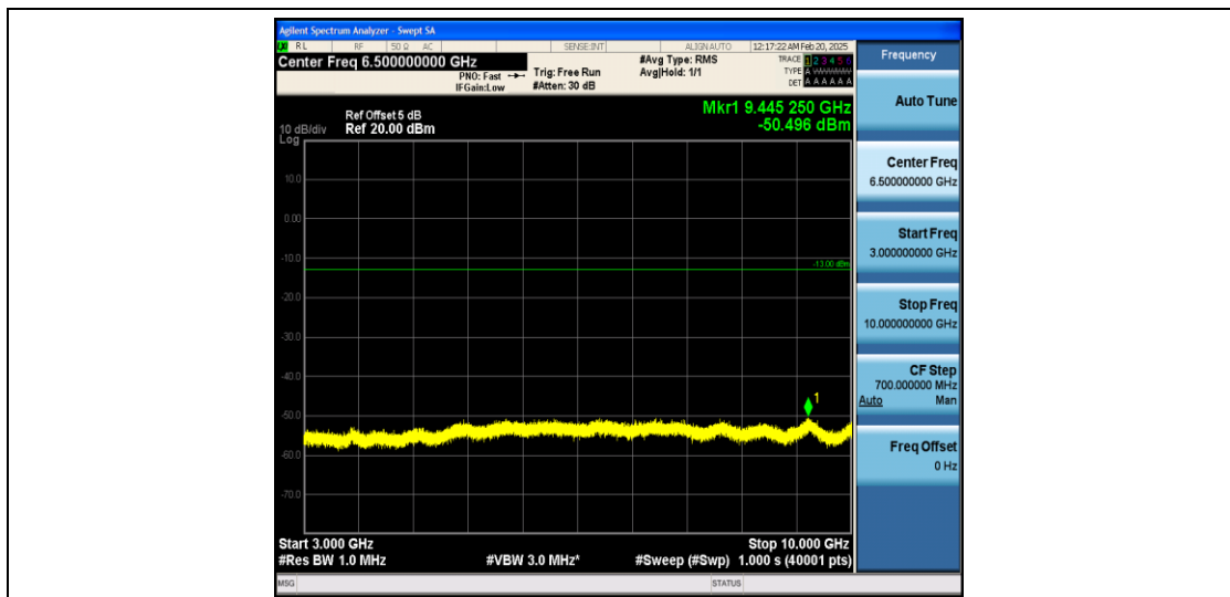
Band12_5MHz_QPSK_23155_1RB#0_3000~10000_3000~10000
