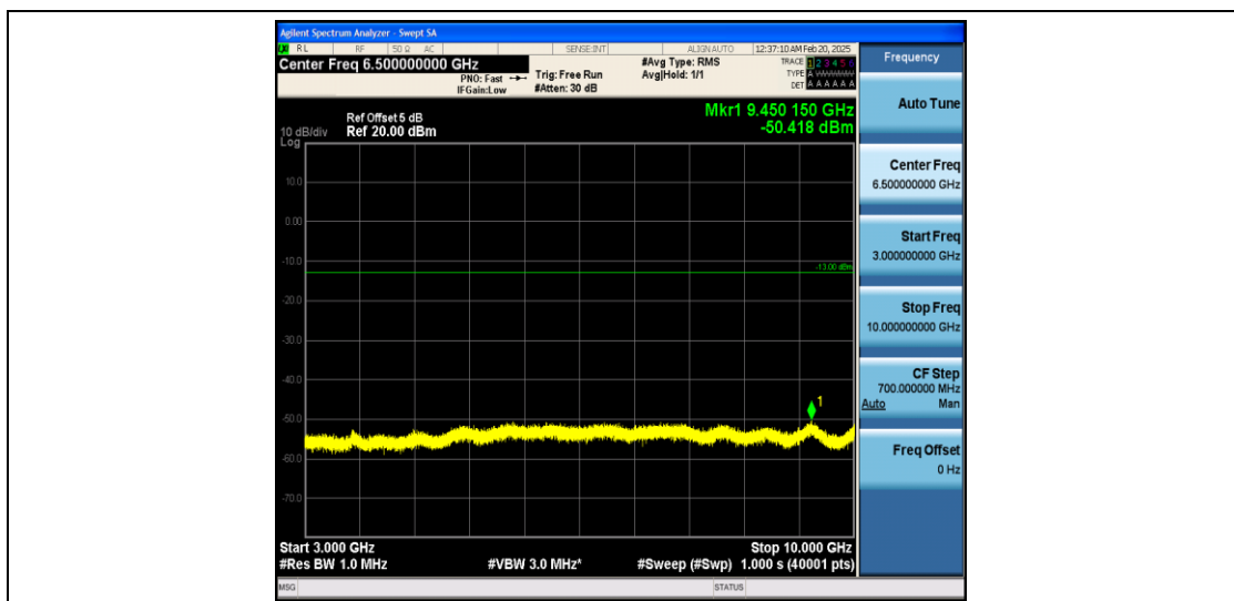
Band12_10MHz_16QAM_23060_1RB#0_3000~10000_3000~10000
