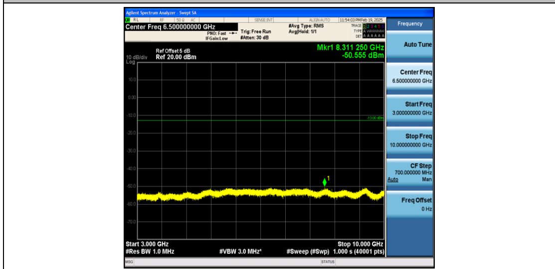
Band12_3MHz_16QAM_23165_1RB#0_3000~10000_3000~10000
