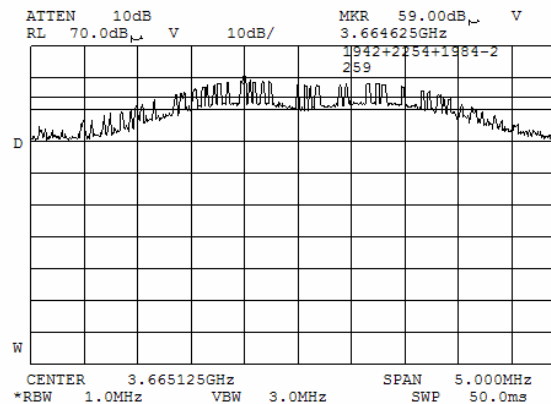
Plot 7.3.80 Radiated emission measurements at the forth harmonic of mid carrier frequency
