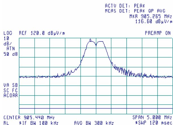
Plot 7.3.2 Field strength measurements at the low carrier frequency
