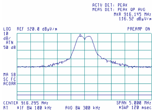
Plot 7.3.4 Field strength measurements at the mid carrier frequency
