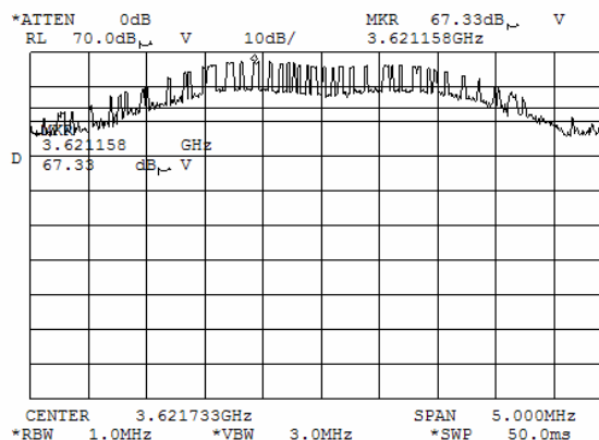
Plot 7.3.76 Radiated emission measurements at the forth harmonic of low carrier frequency
