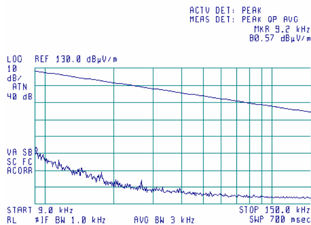
Plot 7.3.14 Radiated emission measurements from 9 to 150 kHz at the mid carrier frequency
