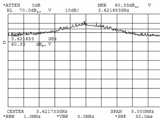
Plot 7.3.74 Radiated emission measurements at the forth harmonic of low carrier frequency
