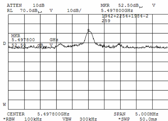
Plot 7.3.102 Radiated emission measurements at the sixth harmonic of mid carrier frequency
