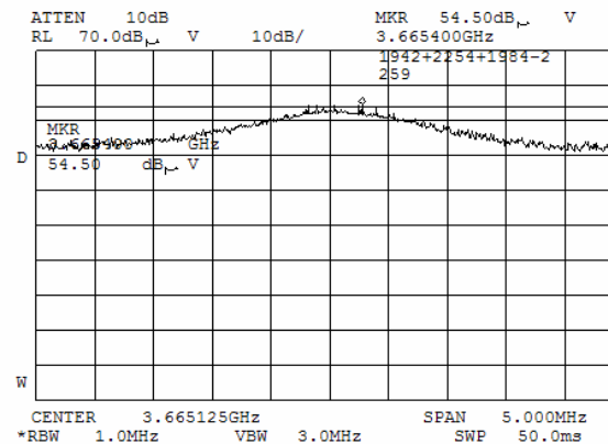
Plot 7.3.78 Radiated emission measurements at the forth harmonic of mid carrier frequency
