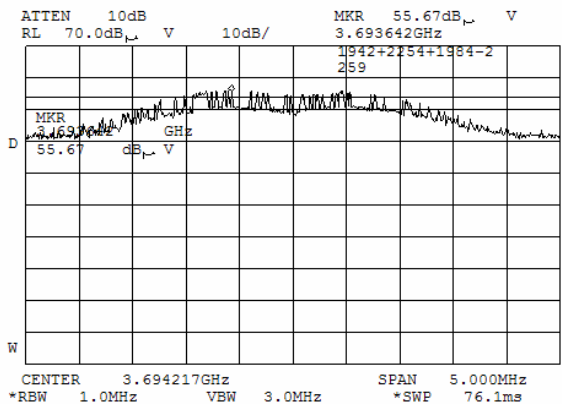
Plot 7.3.84 Radiated emission measurements at the forth harmonic of high carrier frequency
