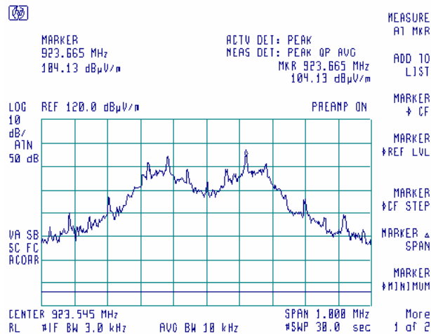
Plot 7.4.12 Peak spectral power density at high frequency zoomed at the peak
