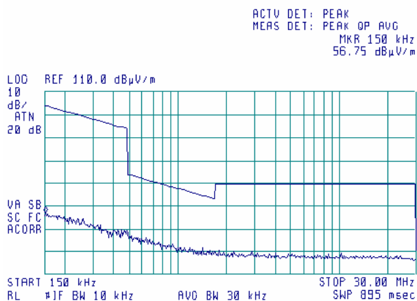
Plot 7.3.22 Radiated emission measurements from 0.15 to 30 MHz at the low carrier frequency
