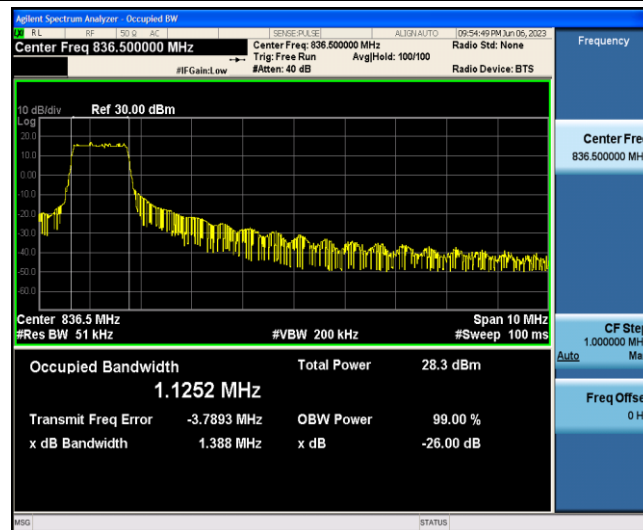
Band5-10MHz-QPSK-20525-6-0-Low-1.1252-1.388-PASS
