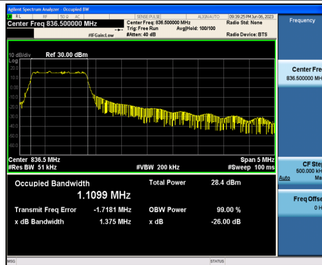
Band5-5MHz-16QAM-20525-6-0-Low-1.1099-1.375-PASS
