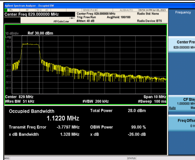
Band5-10MHz-QPSK-20450-6-0-Low-1.1220-1.328-PASS
