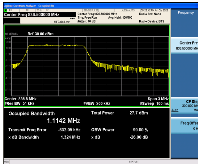
Band5-3MHz-16QAM-20525-6-0-Low-1.1142-1.324-PASS
