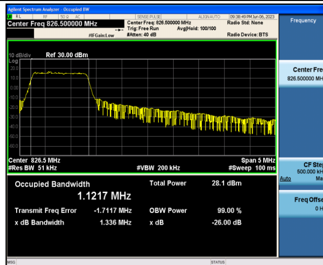
Band5-5MHz-16QAM-20425-6-0-Low-1.1217-1.336-PASS
