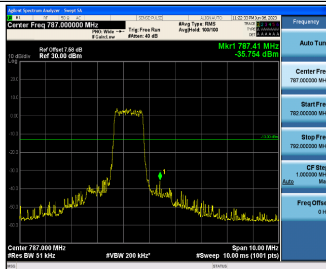
Band13-5MHz-QPSK-23255-6-0-High--35.75-PASS
