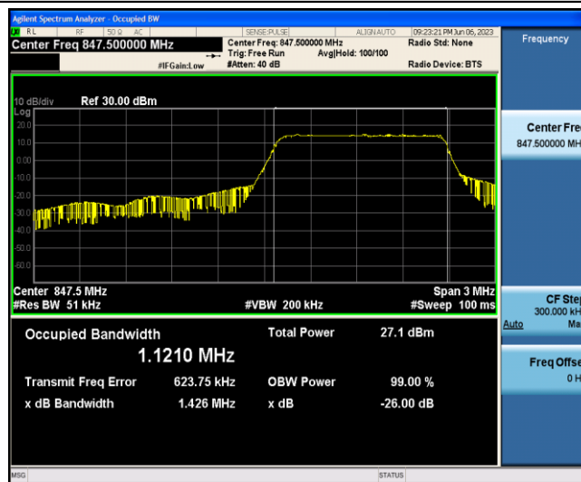
Band5-3MHz-16QAM-20635-6-0-High-1.1210-1.426-PASS
