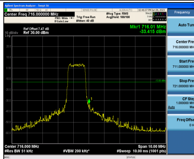
Band12-5MHz-16QAM-23155-6-0-High--33.42-PASS
