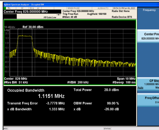
Band5-10MHz-16QAM-20450-6-0-Low-1.1151-1.333-PASS
