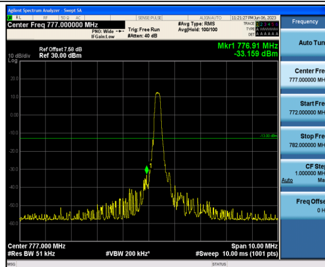
Band13-5MHz-QPSK-23205-1-0-Low--33.16-PASS
