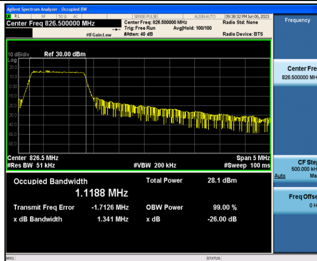
Band5-5MHz-QPSK-20425-6-0-Low-1.1188-1.341-PASS
