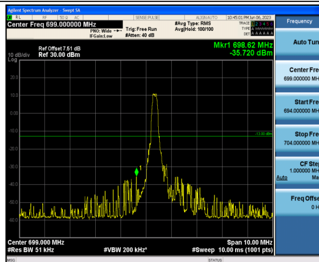
Band12-5MHz-16QAM-23035-1-0-Low--35.72-PASS
