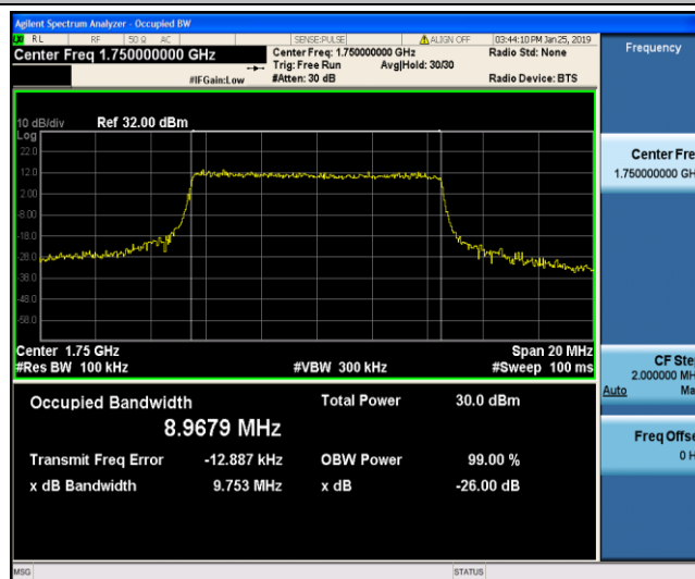
Band4_10MHz_QPSK_175000_50RB#0
