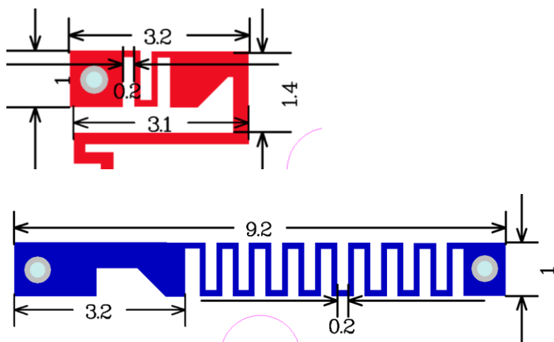
Antenna Photo & Length(mm)
