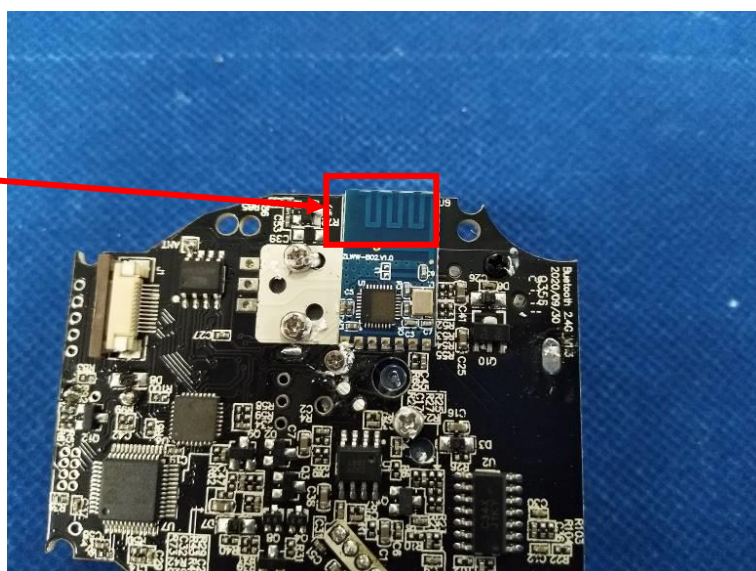
Bluetooth Antenna
