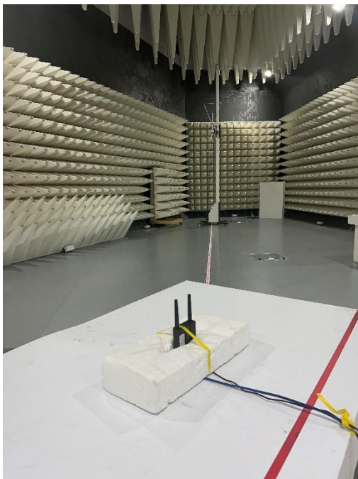
Photograph 1: View Test Set Up Radiated Emissions 30 – 1000 MHz
