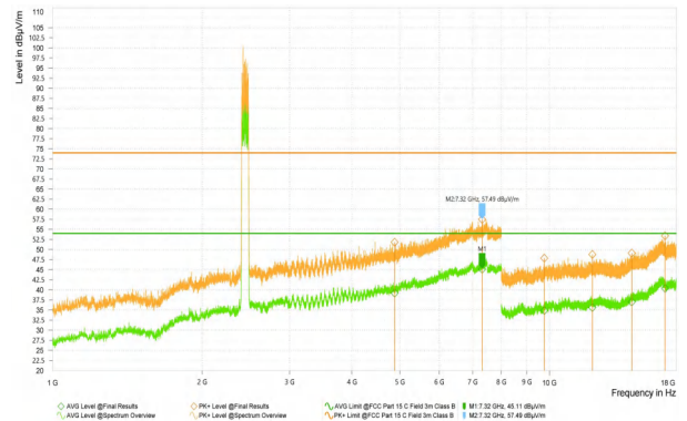
BLE_1M_2440_Low
