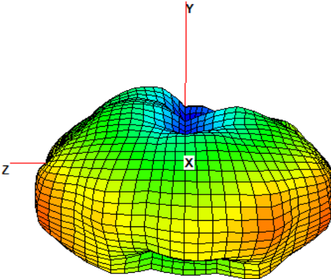
2.44GHz Y-Z plane View
