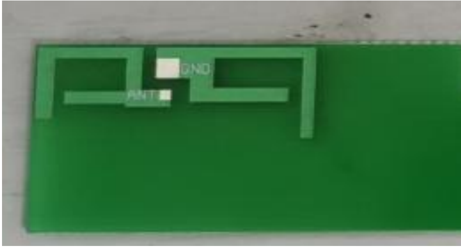
ANT 2(Wi-Fi)
