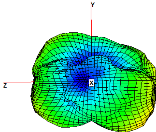
Band1-5.200GHz Y-Z plane View
