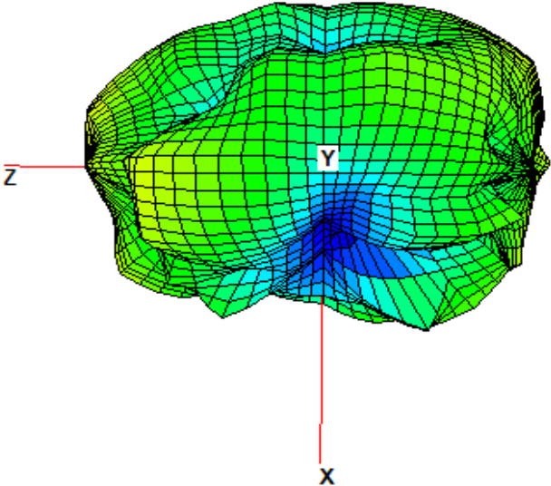
Band4-5.800GHz X-Z plane View
