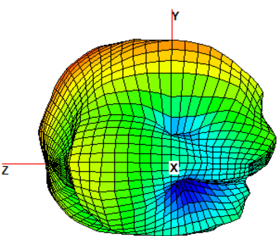
2.44GHz Y-Z plane View
