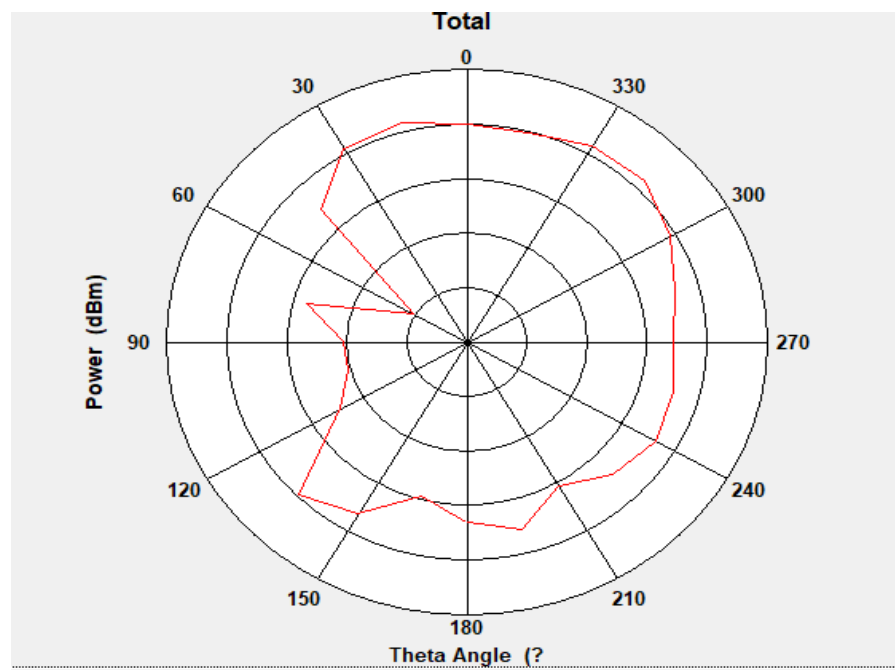
Band4-5.800GHz Y-Z plane View
