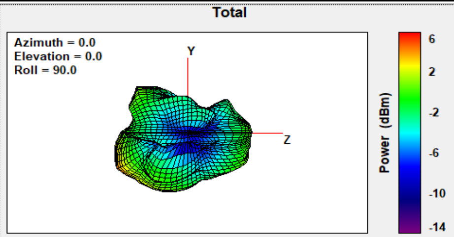
2.44GHz Y-Z View
