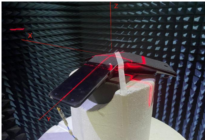
Band4-5.800GHz Y-Z View
