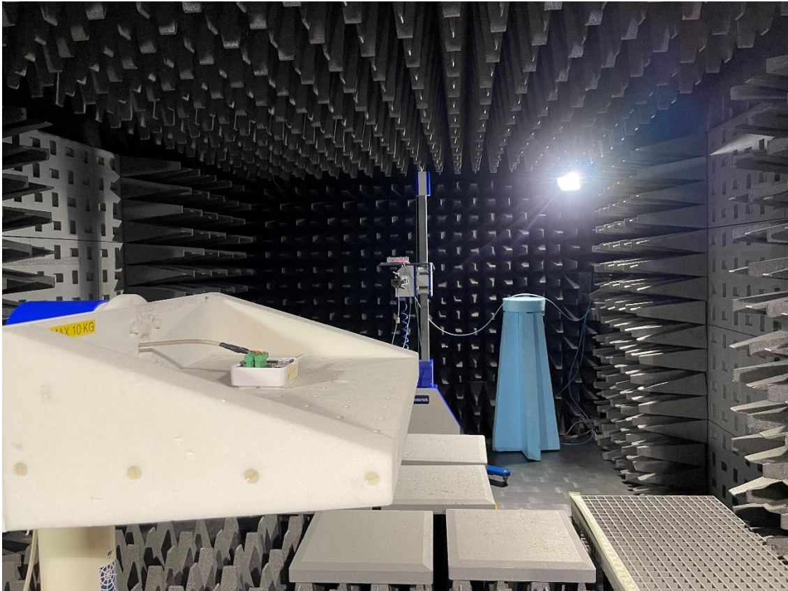
Photo of the test set-up for radiated emission 13 - 18 GHz
