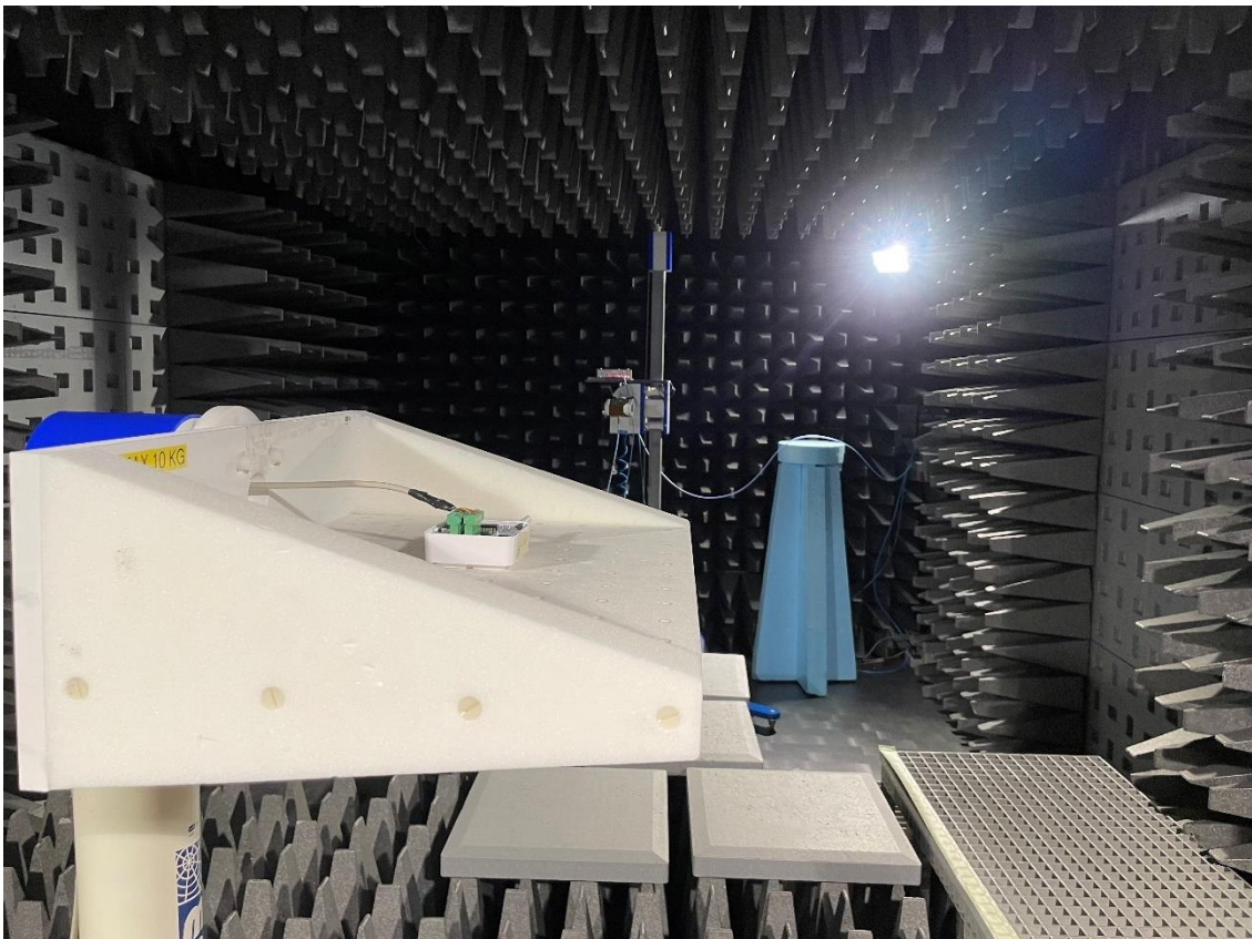
Photo of the test set-up for radiated emission 18 - 26.5 GHz
