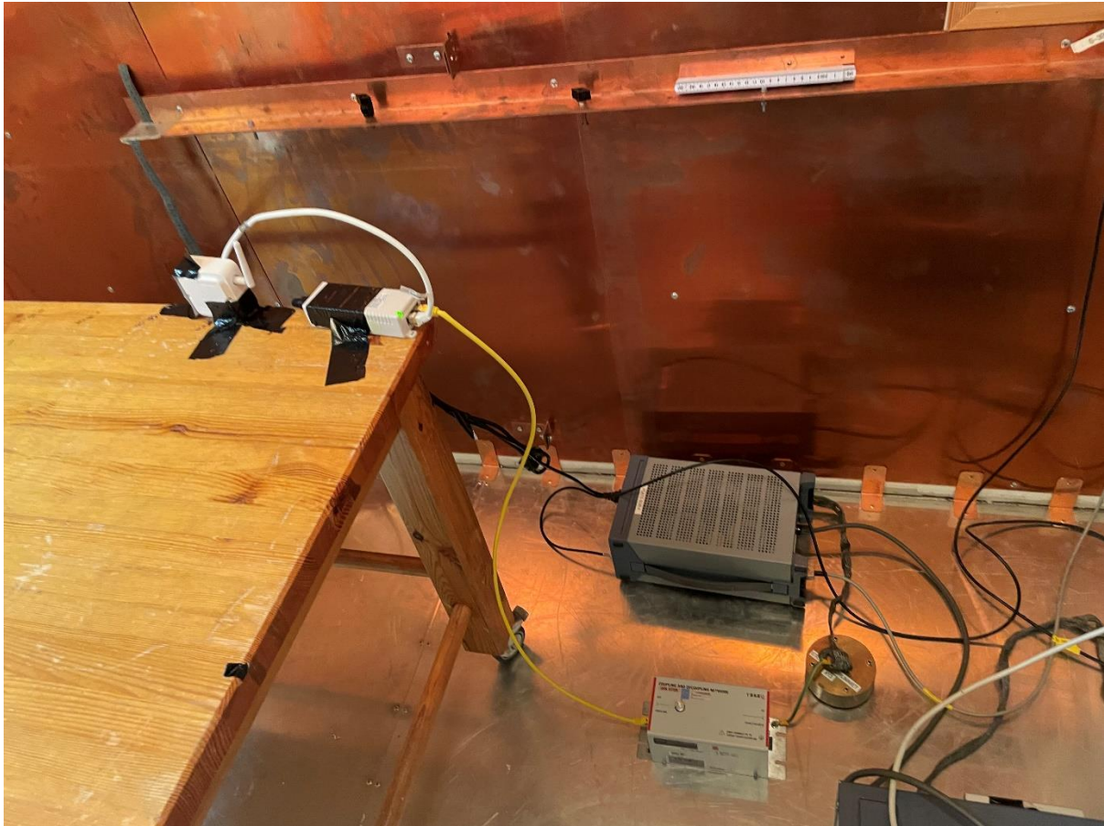
Photo of the test set-up for conducted emission 0.15MHz - 30MHz
