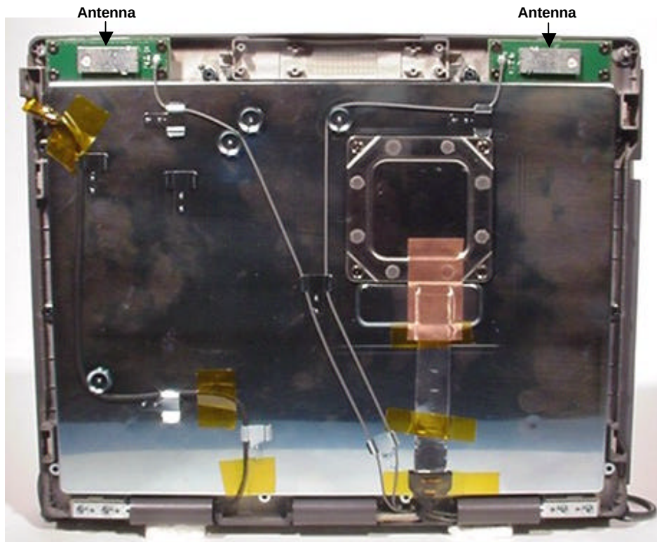
Back Side of LCD Display
