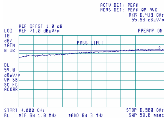
Plot 7.5.30 Radiated emission measurements from 4000 to 6500 MHz at the high carrier frequency
