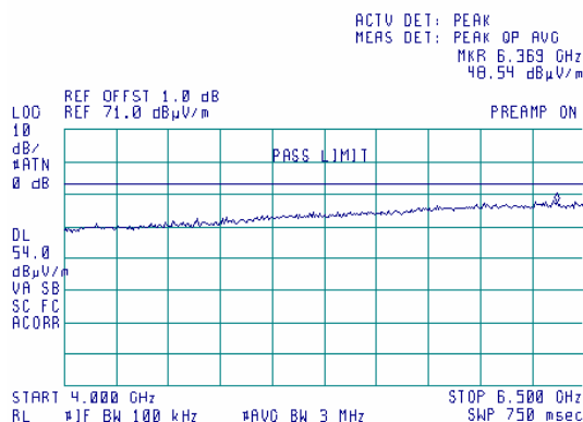
Plot 7.5.32 Radiated emission measurements from 4000 to 6500 MHz at the mid carrier frequency
