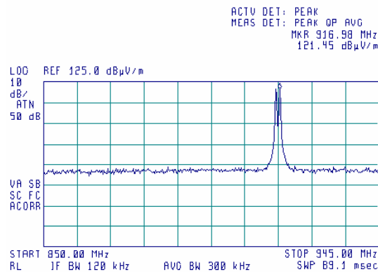
Plot 7.5.92 Radiated emission measurements from 850 to 945 MHz at the high carrier frequency
