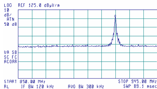
Plot 7.5.18 Radiated emission measurements from 850 to 945 MHz at the high carrier frequency
