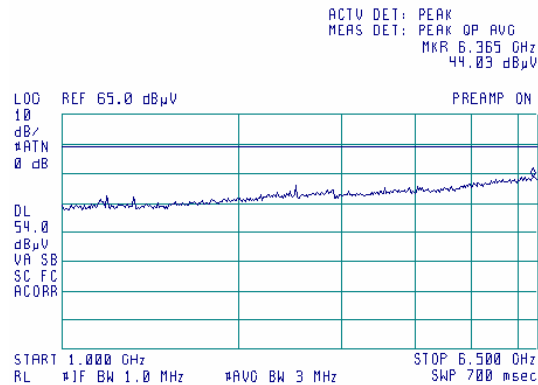
Plot 8.2.5 Radiated emission measurements above 1000 MHz, vertical and horizontal antenna polarization, mid frequency channel
