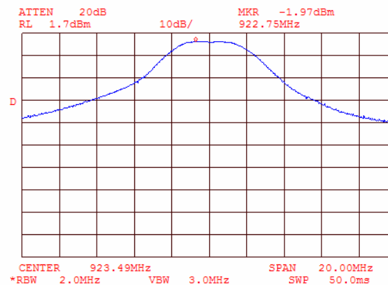
Plot 7.2.6 Peak output power at high frequency
