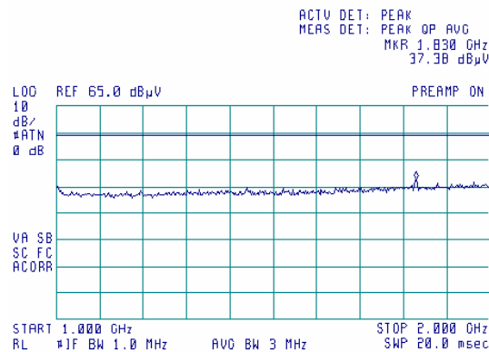
Plot 7.5.24 Radiated emission measurements from 1000 to 2000 MHz at the high carrier frequency
