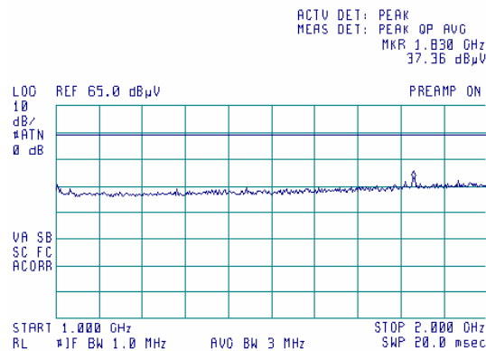
Plot 7.5.98 Radiated emission measurements from 1000 to 2000 MHz at the high carrier frequency
