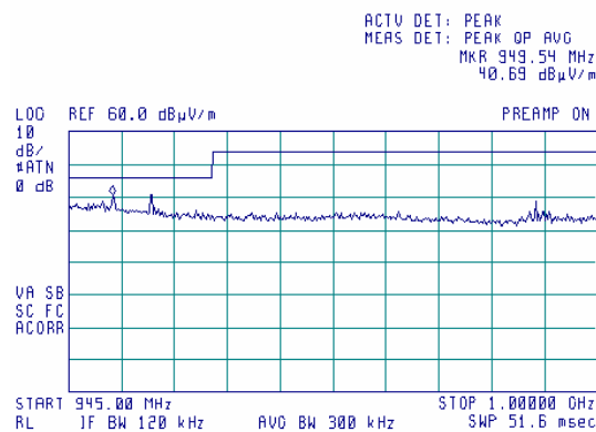
Plot 7.5.94 Radiated emission measurements from 945 to 1000 MHz at the mid carrier frequency
