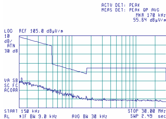
Plot 7.5.86 Radiated emission measurements from 0.15 to 30 MHz at the high carrier frequency
