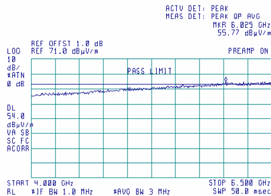
Plot 7.5.104 Radiated emission measurements from 4000 to 6500 MHz at the high carrier frequency
