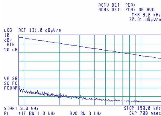
Plot 7.5.82 Radiated emission measurements from 9 to 150 kHz at the mid carrier frequency
