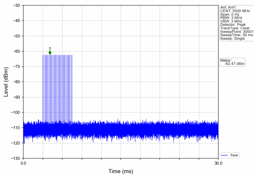
Signal Calibration_802.11a_2C_5500MHz_RadarType3_Trial0
