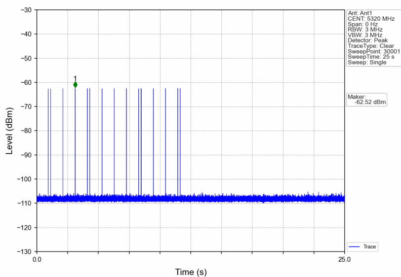
Signal Calibration_802.11a_2A_5320MHz_RadarType5_Trial0
