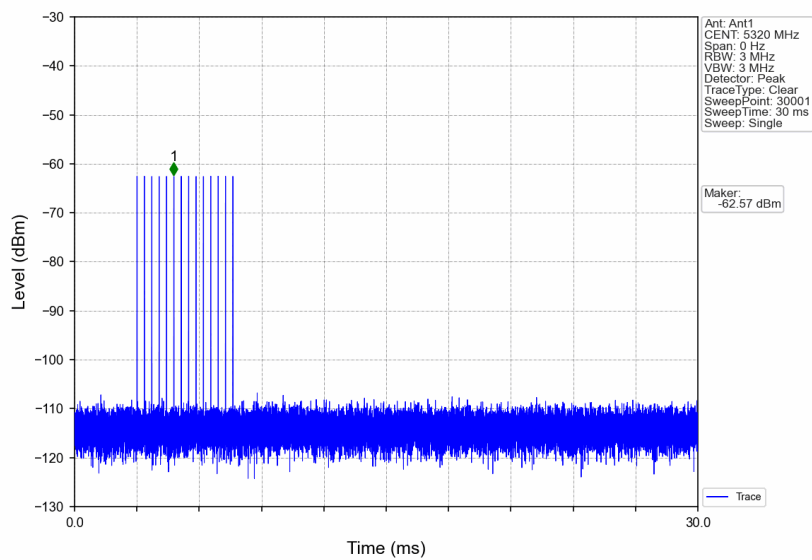
Signal Calibration_802.11a_2A_5320MHz_RadarType5_Trial0
