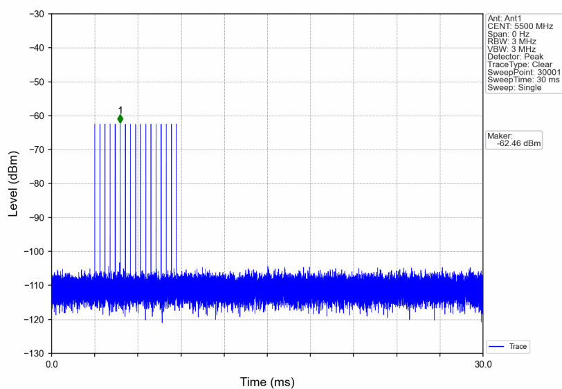
Signal Calibration_802.11a_2C_5500MHz_RadarType3_Trial0
