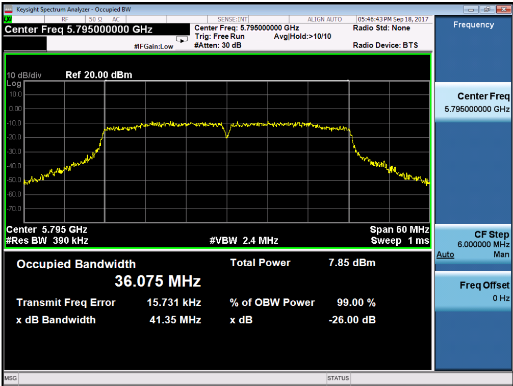
TEST PLOT OF BANDWIDTH FOR 5795MHz
