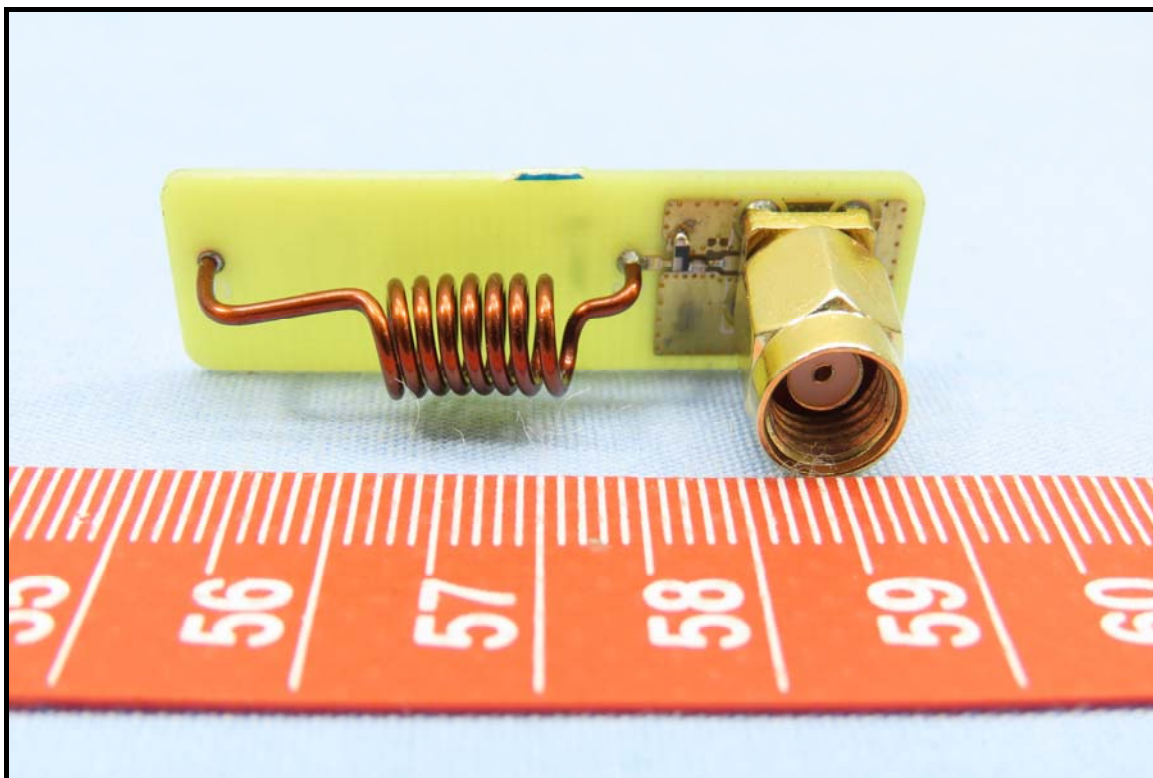
Antenna 4 (Brand: SolarEdge, PN: AS4035-1)
