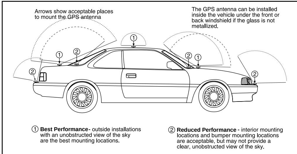
Figure 2.5 Antenna Mounting Locations for Automobile
