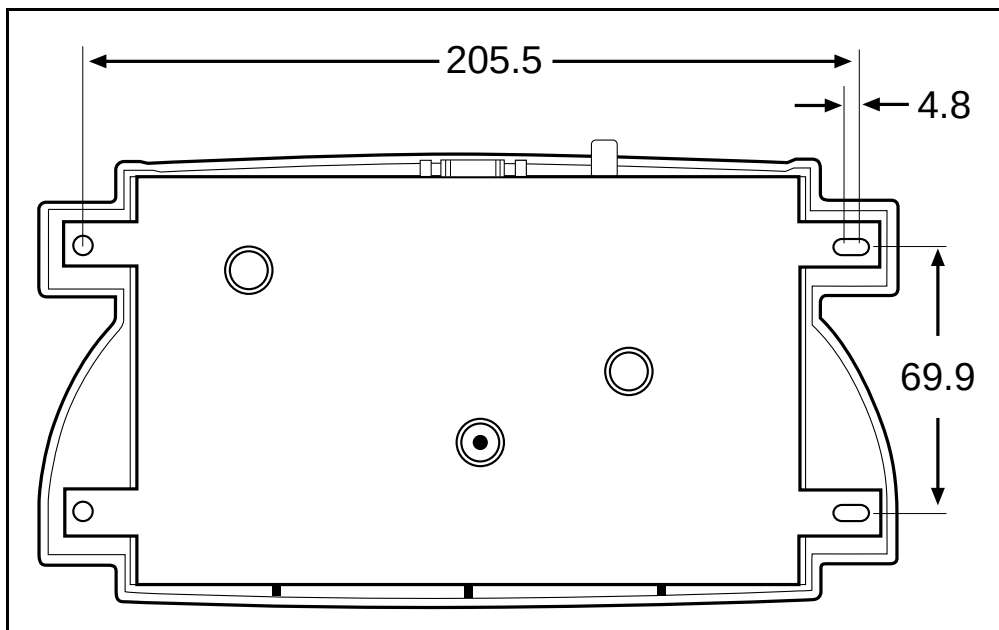
Figure 2.4 CrossCheck CDPD Mounting Dimensions (in millimeters)
