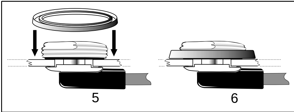
Figure 2.17 Attaching the Antenna to the Cable Assembly
