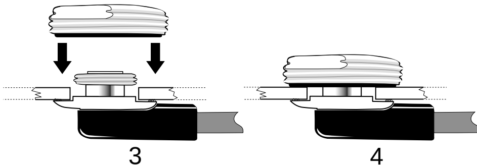
Figure 2.16 Re-installing the Brass Nut
