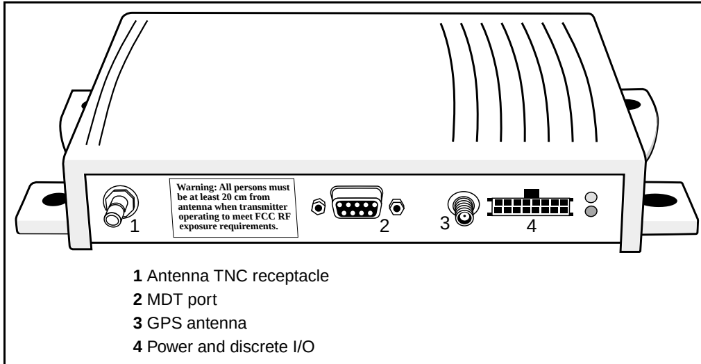
Figure 2.1 CrossCheck CDPD Connections
