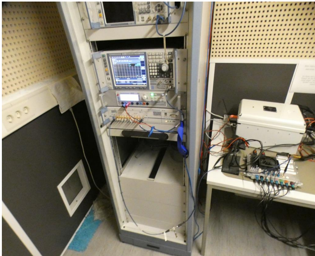
Photo 1: Test setup for conducted measurements
