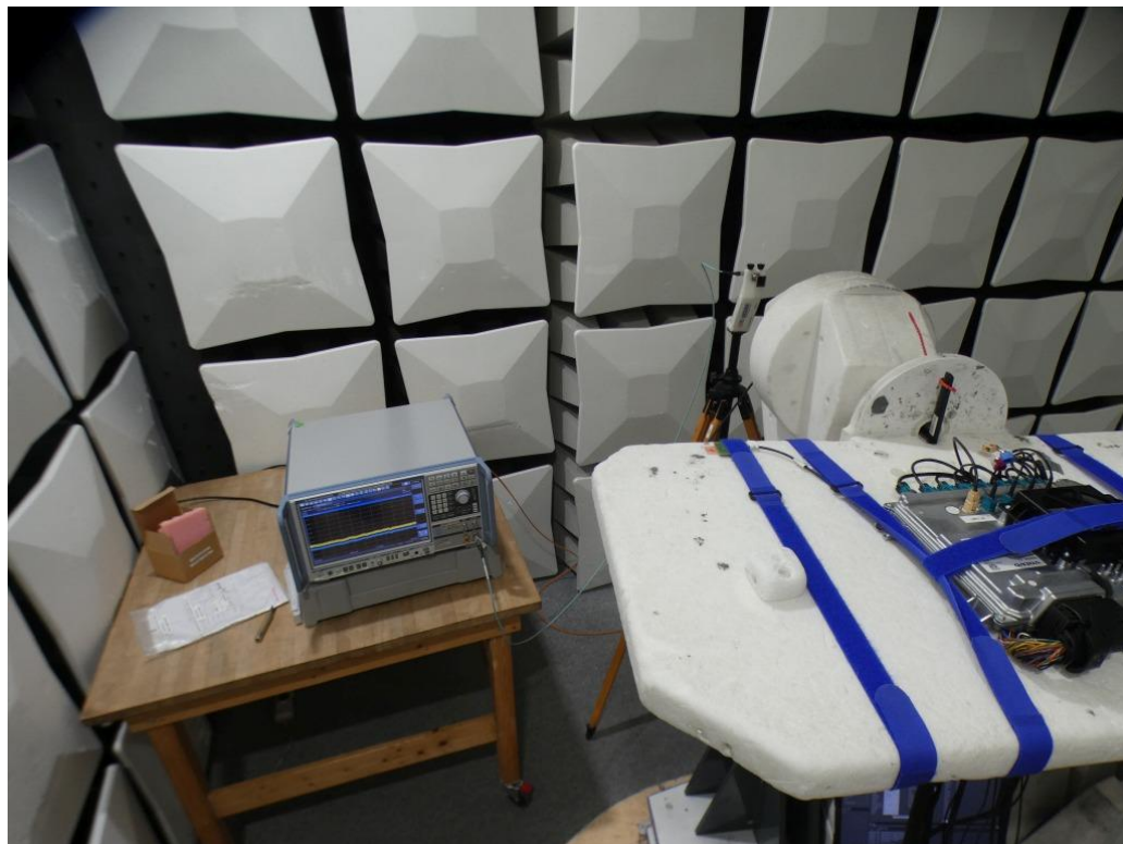
Photo 8: Test setup for radiated measurements above 26 GHz
