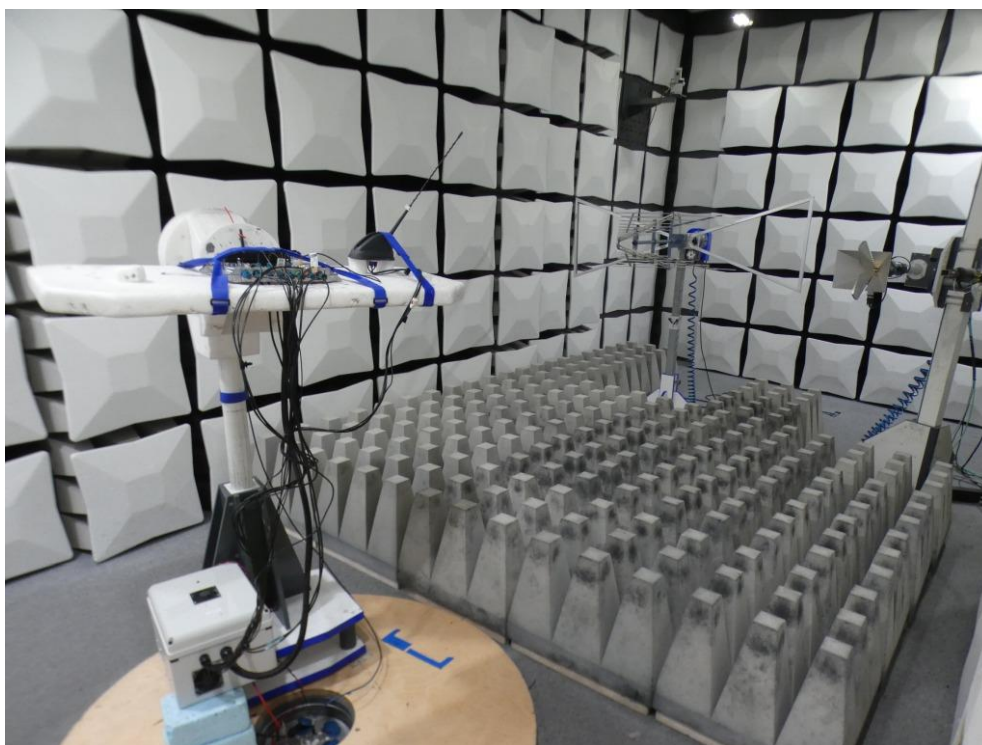
Photo 6: Test setup for radiated measurements above 1 GHz
