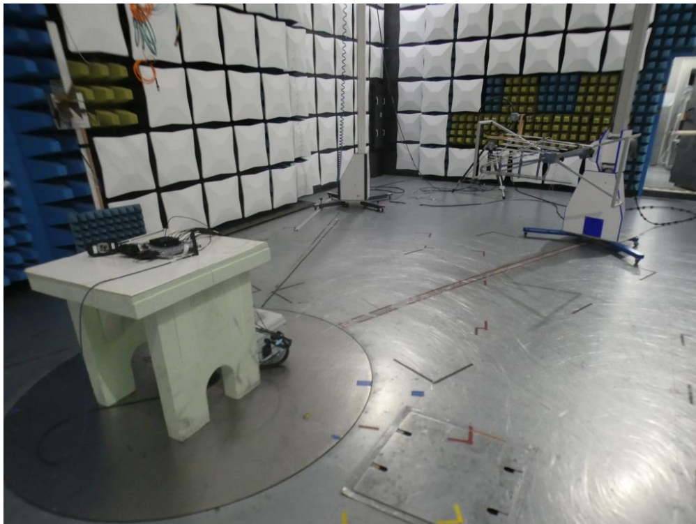
Photo 3: Test setup for radiated measurements below 1 GHz
