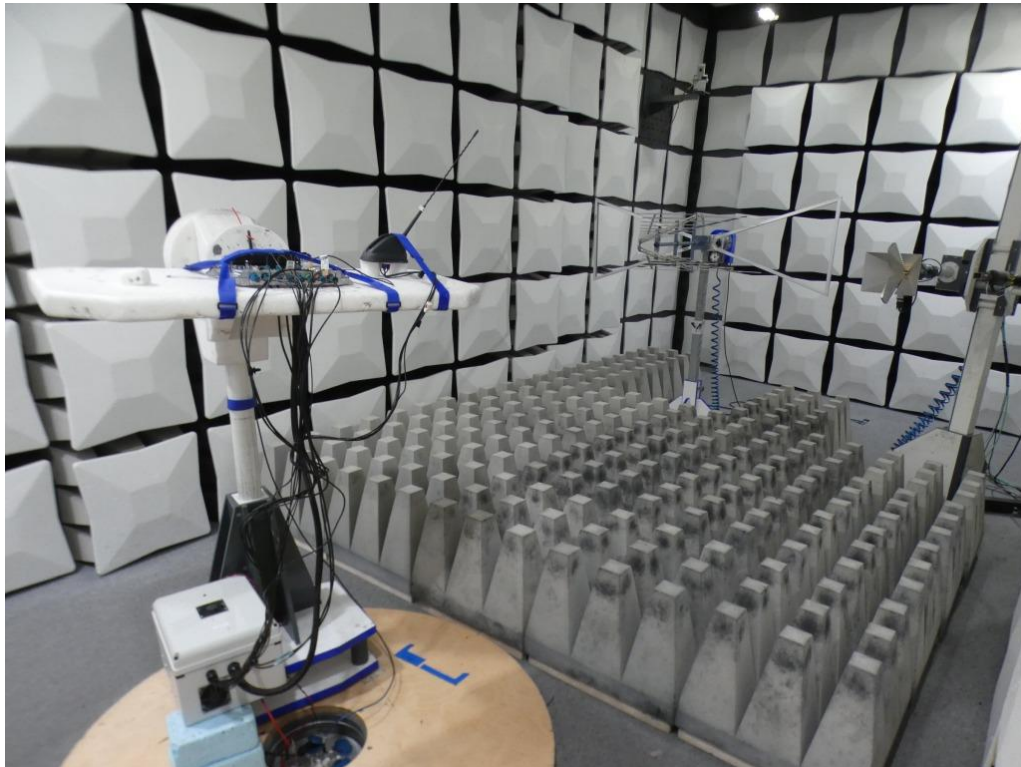
Photo 7: Test setup for radiated measurements above 18 GHz, FCC15b
