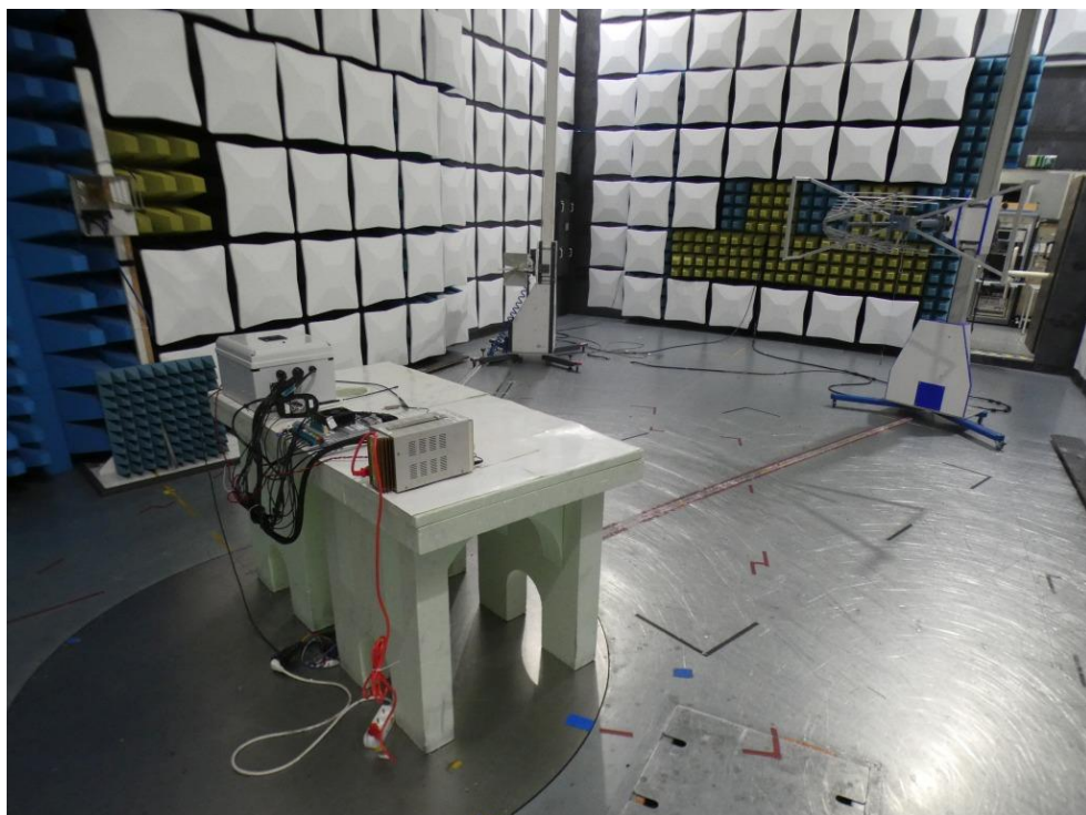
Photo 4: Test setup for radiated measurements below 1 GHz, FCC15b
