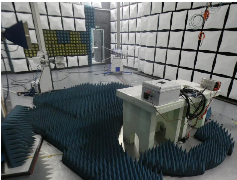
Photo 5: Test setup for radiated measurements above 1 GHz, FCC15b
