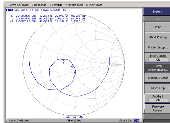
Smith Chart(S 11 )
