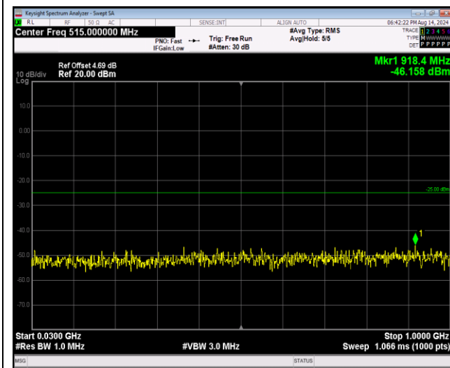
Band41-20MHz-64QAM-40620-1RB#0-Range1:30~1000MHz
