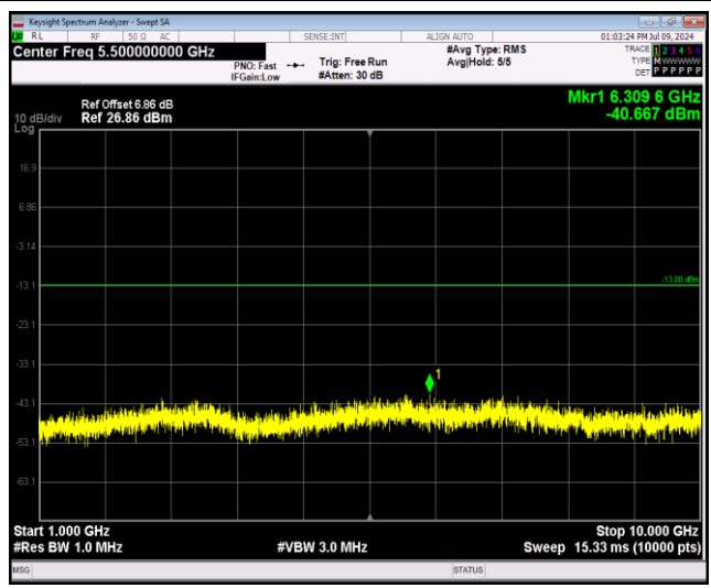
Band26-15MHz-16QAM-26965-1RB#0-Range2:1000~10000MHz
