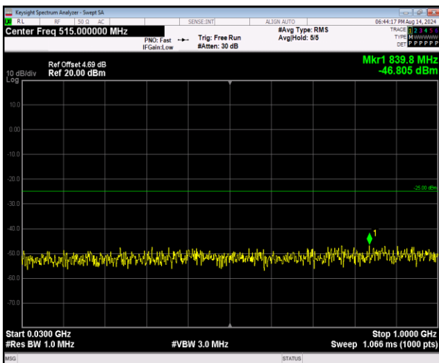
Band66-1.4MHz-QPSK-131979-1RB#0-Range1:30~1000MHz
