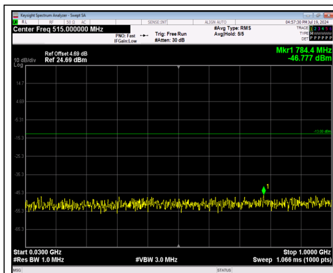
Band66-1.4MHz-QPSK-132665-1RB#0-Range1:30~1000MHz
