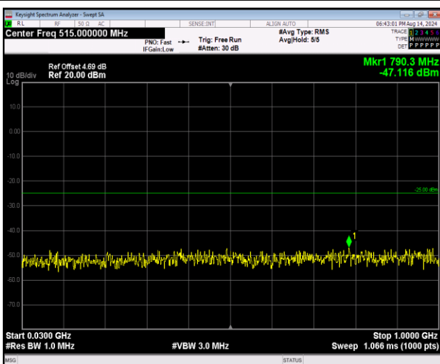
Band41-20MHz-16QAM-41490-1RB#0-Range1:30~1000MHz
