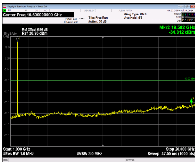
Band66-1.4MHz-16QAM-132665-1RB#0-Range2:100 0~20000MHz
