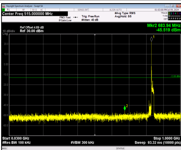
Band26-15MHz-16QAM-26865-1RB#0-Range1:30~1000MHz
