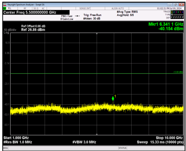
Band26-15MHz-16QAM-26965-1RB#0-Range2:1000~10000MHz
