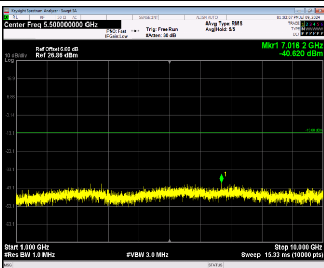
Band26-15MHz-16QAM-26865-1RB#0-Range2:1000~10000MHz
