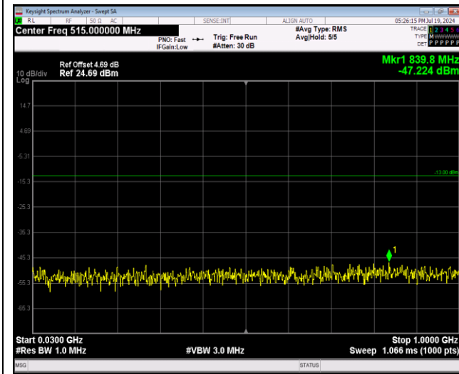
Band66-20MHz-16QAM-132322-1RB#0-Range1:30 ~1000MHz
