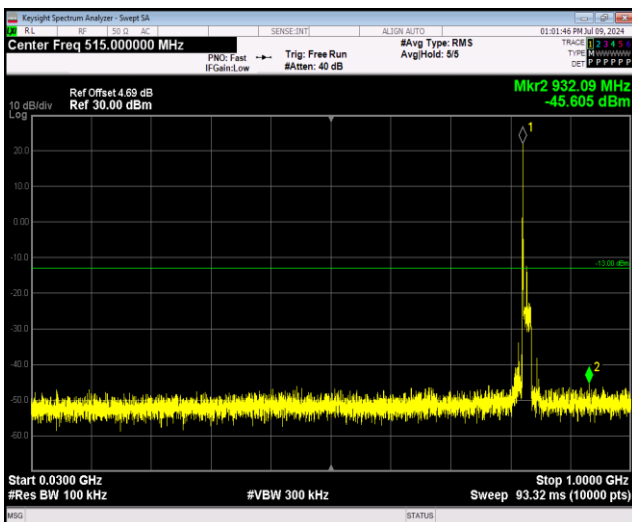
Band26-15MHz-64QAM-26915-1RB#0-Range1:30~1000MHz
