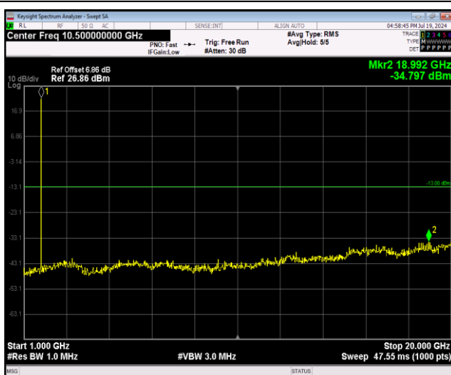
Band66-1.4MHz-64QAM-131979-1RB#0-Range2:100 0~20000MHz
