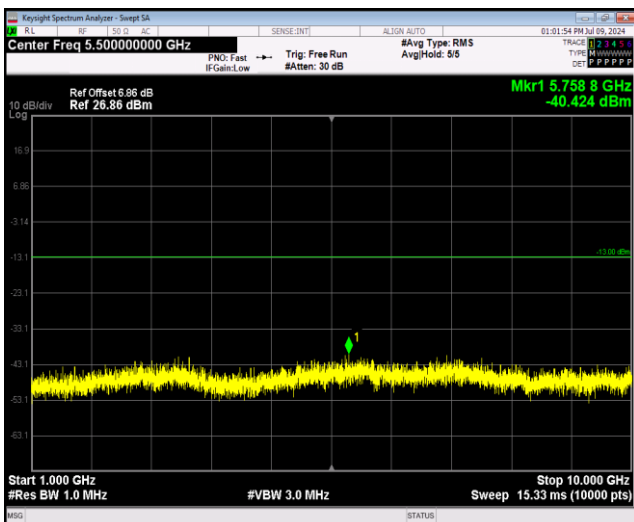
Band26-15MHz-64QAM-26915-1RB#0-Range2:1000~10000MHz
