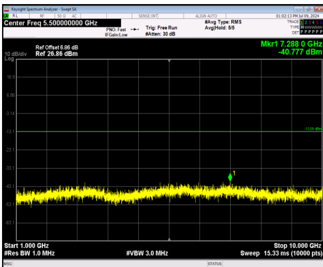
Band26-15MHz-QPSK-26965-1RB#0-Range2:1000~10000MHz
