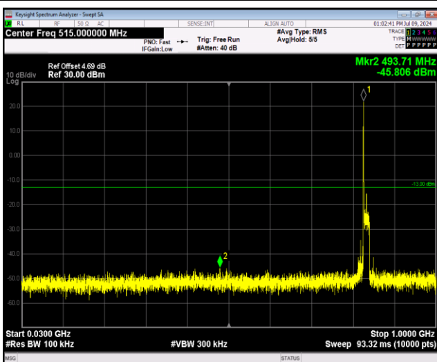
Band26-15MHz-64QAM-26965-1RB#0-Range1:30~1000MHz
