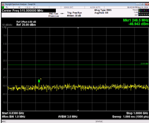
Band41-20MHz-16QAM-40620-1RB#0-Range1:30~1000MHz
