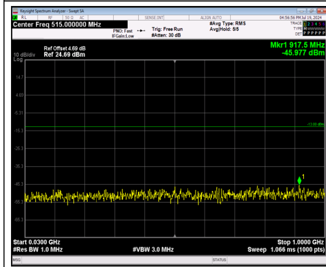
Band66-1.4MHz-16QAM-131979-1RB#0-Range1:3~0~1000MHz
