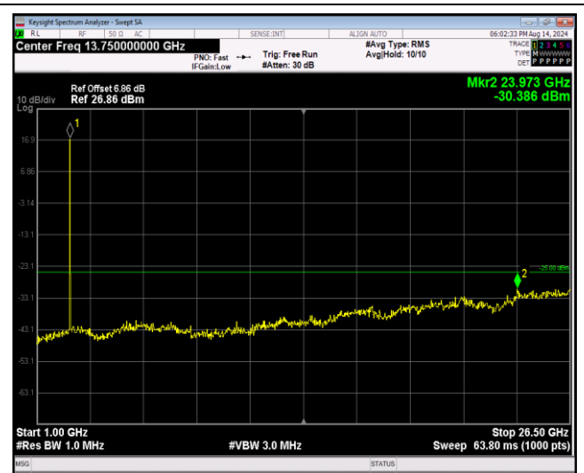
Band41-5MHz-16QAM-41565-1RB#0-Range2:1000~26500MHz
