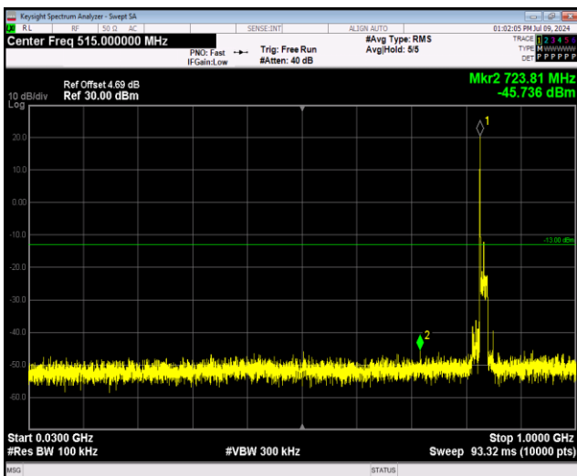
Band26-15MHz-QPSK-26965-1RB#0-Range1:30~1000MHz
