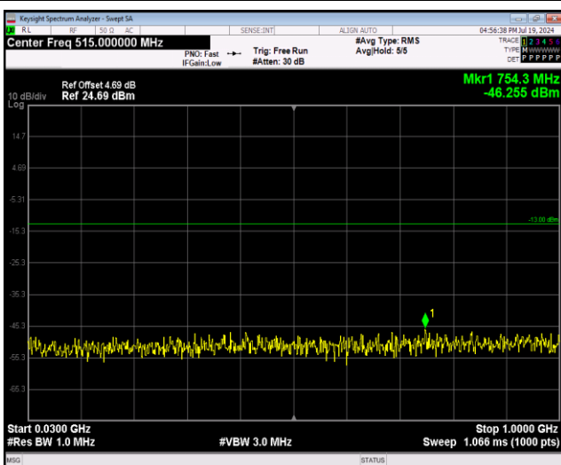
Band66-1.4MHz-QPSK-132322-1RB#0-Range1:30~1000MHz
