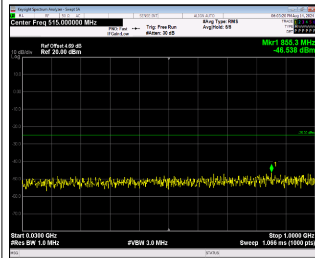
Band41-5MHz-64QAM-39675-1RB#0-Range1:30~1000MHz
