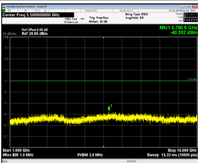
Band26-15MHz-64QAM-26965-1RB#0-Range2:1000~10000MHz
