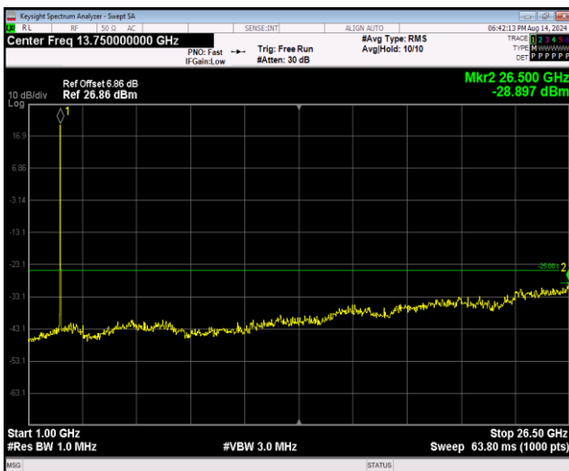
Band41-20MHz-16QAM-40620-1RB#0-Range2:1000~26500MHz
