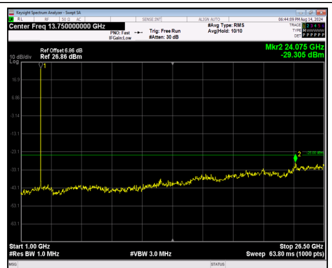
Band41-20MHz-64QAM-39750-1RB#0-Range2:1000~26500MHz
