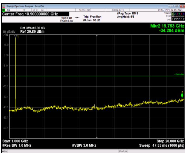
Band66-1.4MHz-QPSK-132322-1RB#0-Range2:1000~20000MHz
