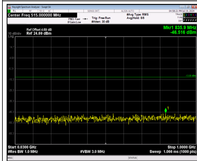
Band66-1.4MHz-16QAM-131979-1RB#0-Range1:3~0~1000MHz
