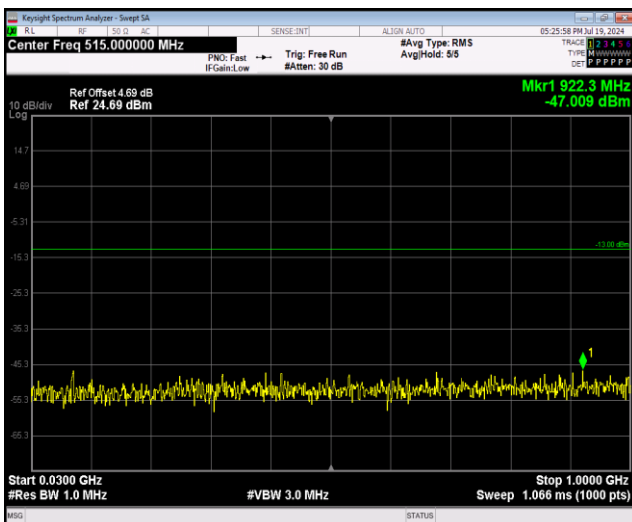
Band66-20MHz-QPSK-132322-1RB#0-Range1:30~1000MHz
