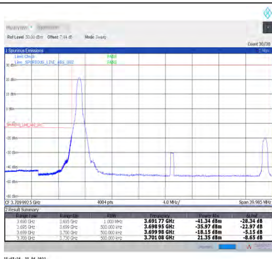
1-N77-3700-3980--30-30-L-1-DFT-PI2BPSK-Edge_1R_B_Left-1@0-Ant1-PASS-see graph
