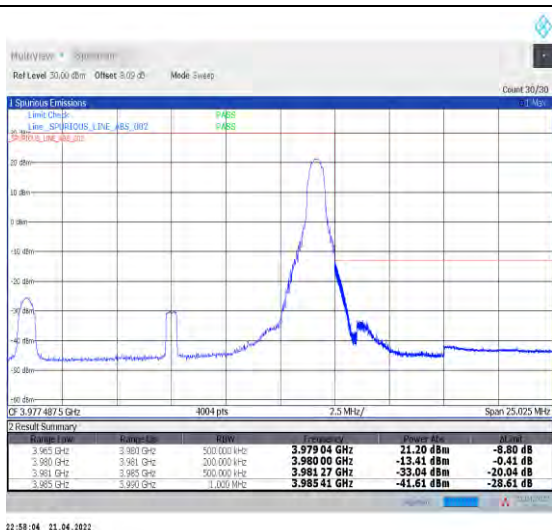
1-N77-3700-3980--30-15-H-2-DFT-PI2BPSK-Edge_1R_B_Right-1@37-Ant1-PASS-see graph
