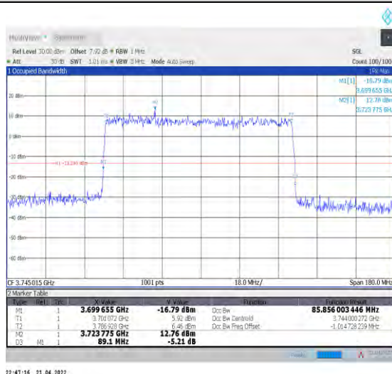
1-N77-3700-3980--30-90-L-5-DFT-256QAM-Outer_Full-240@0-Ant1-85.856-89.100-≤90-PASS
