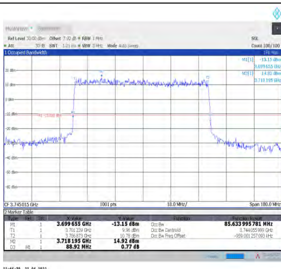
1-N77-3700-3980--30-90-L-2-DFT-PI2BPSK-Outer_Full-240@0-Ant1-85.634-88.920-≤90-PASS
