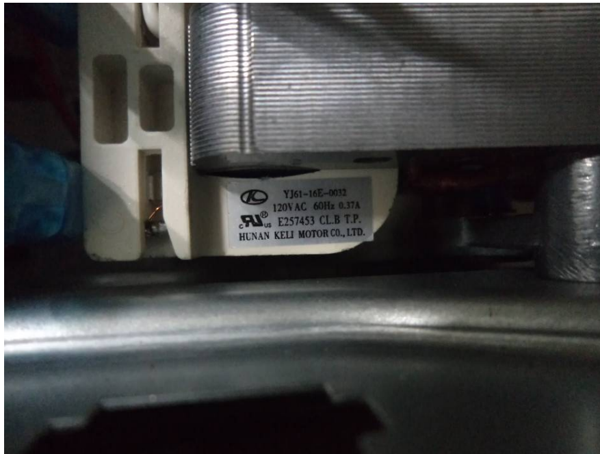
EUT –Motor 1 Label View
