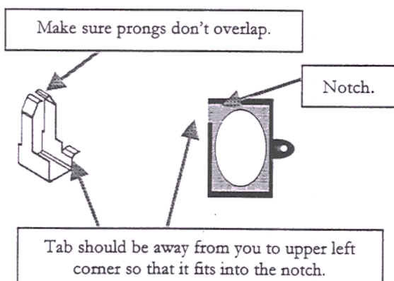
Image 9: Drawings of pronged battery contact and hole to place it in.
