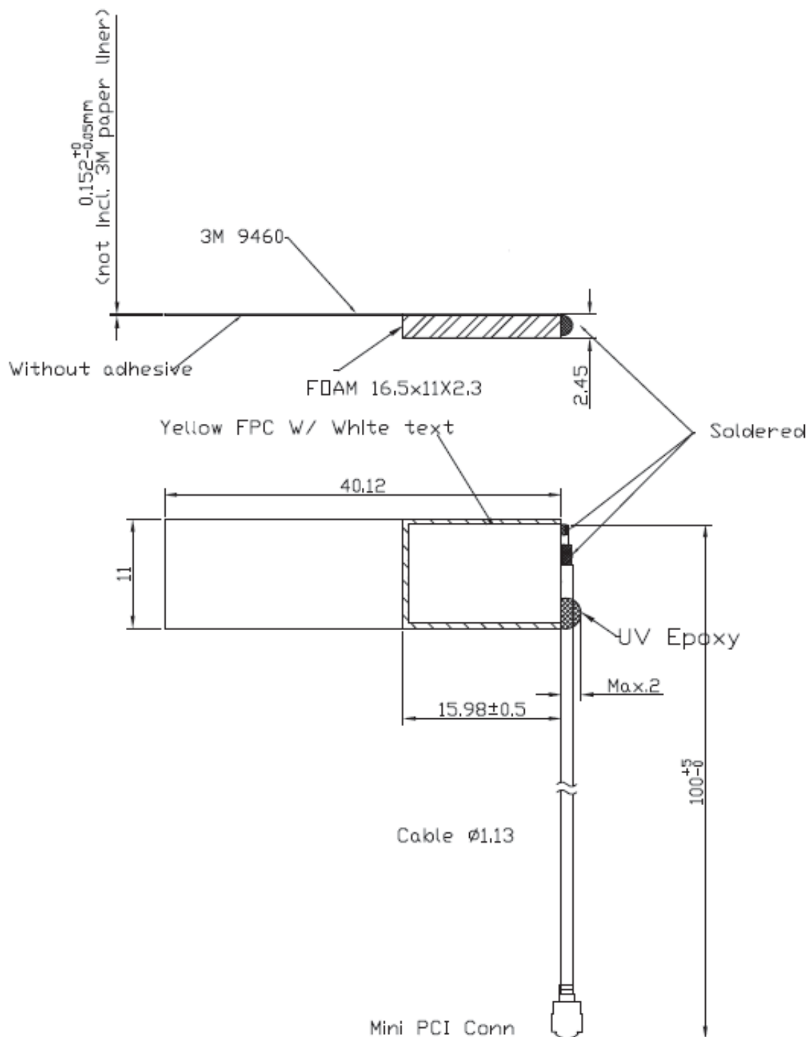
Figure 1 Physical Dimensions
