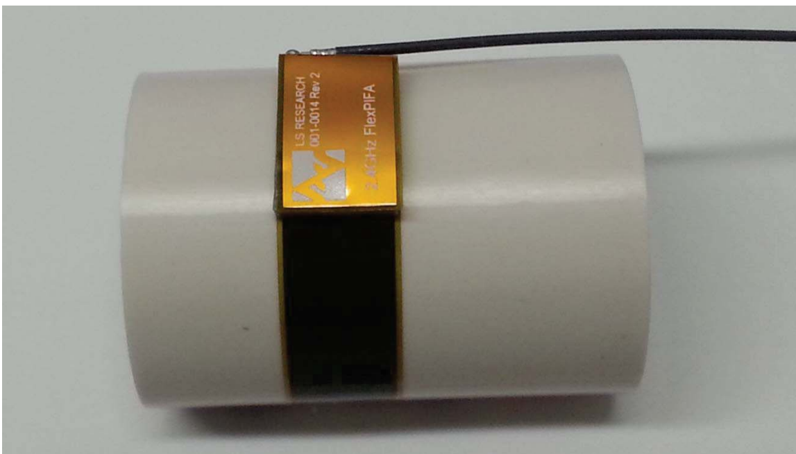
Figure 21 Convex Mounted
