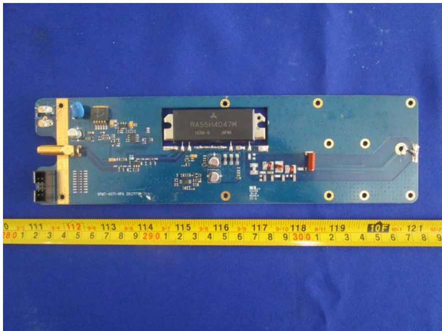
EUT –PA Board Board Top Unshielded View
