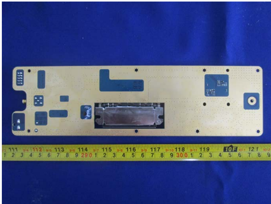
EUT –PA Board Board Bottom View
