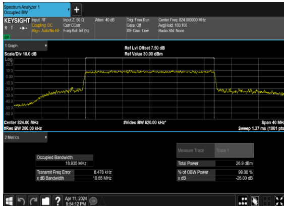
N26(20M)_CP-OFDM_16 QAM_Outer_Full_Mid_CH
