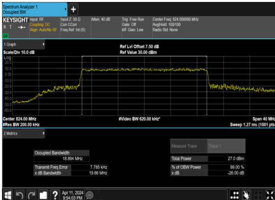
N26(20M)_CP- OFDM_QPSK_Outer_Full_Mid_CH
