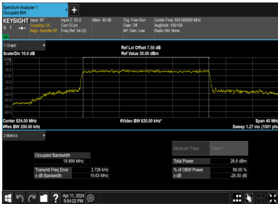
N26(20M)_CP-OFDM_64 QAM Outer Full Mid CH
