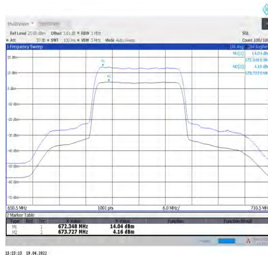
1-N71--15-20-M-2-CP-256QAM-Outer_Full-106@0-Ant1-9.88-100%-0.00-9.88-PASS-≤13
