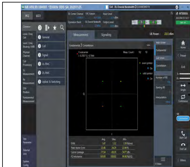
1-N71--15-20-M-1-DFT-PI2BPSK-Outer_Full-100@0-A Ant1-see graph-PASS
