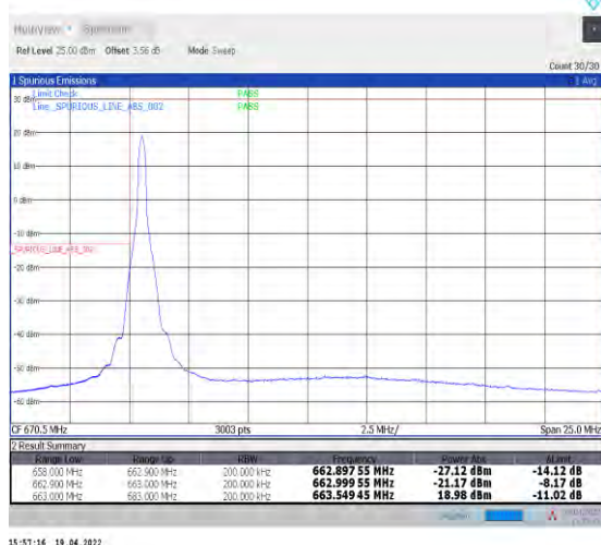
1-N71--15-20-L-4-CP-QPSK-Edge_1RB_Left-1@0-Ant1-PASS-see graph
