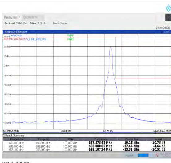
1-N71--15-10-H-2-DFT-PI2BPSK-Edge_1RB_Right-1@51-Ant1-PASS-see graph
