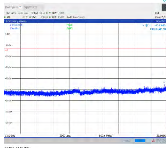
1-N71--15-20-L-1-DFT-PI2BPSK-Inner_1RB_Left-1@ 1-12000-20000-Ant1--46.79--13-PASS
