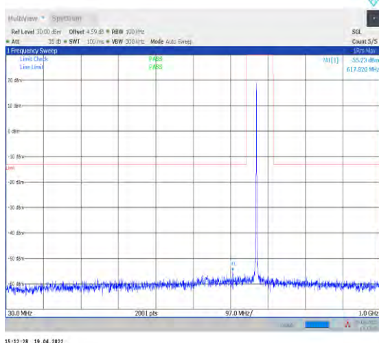
1-N71--15-20-H-1-DFT-PI2BPSK-Inner_1RB_Left-1 @1-30-1000-Ant1--55.23--13-PASS
