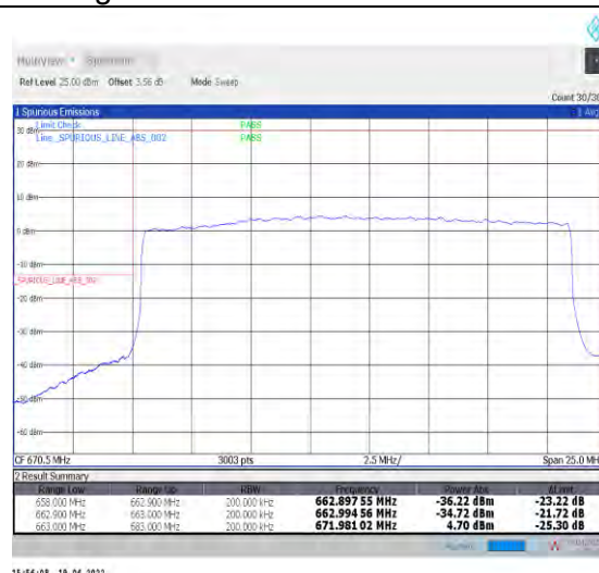
1-N71--15-20-L-3-DFT-PI2BPSK-Outer_Full-100@0-Ant1-PASS-see graph
