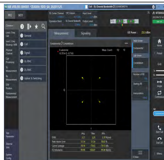
1-N71--15-20-M-2-DFT-QPSK-Outer_Full-100@0-A nt1-see graph-PASS
