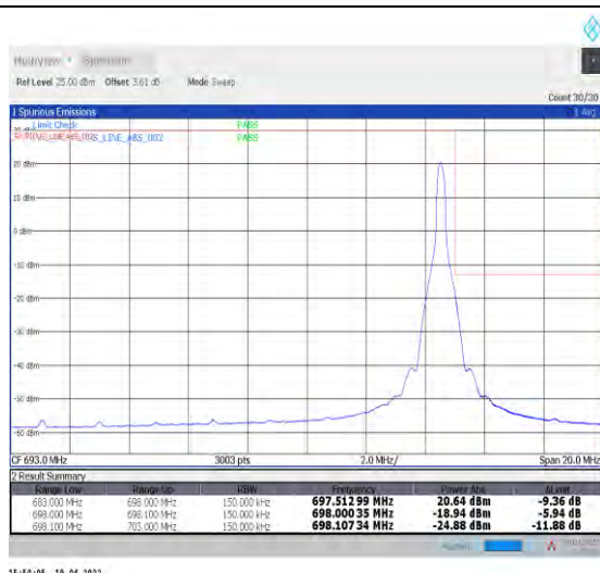
1-N71--15-15-H-2-DFT-PI2BPSK-Edge_1RB_Right-1@78-Ant1-PASS-see graph
