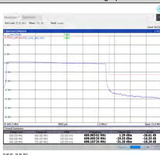
1-N71--15-10-H-6-CP-QPSK-Outer_Full-52@0-Ant1-PASS-see graph
