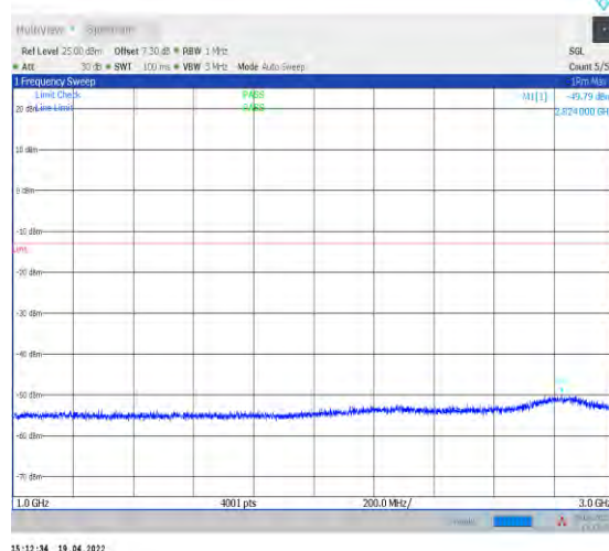
1-N71--15-20-H-1-DFT-PI2BPSK-Inner_1RB_Left-1 @1-1000-3000-Ant1--49.79--13-PASS
