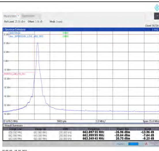
1-N71--15-20-L-1-DFT-PI2BPSK-Edge_1RB_Left-1@0-Ant1-PASS-see graph
