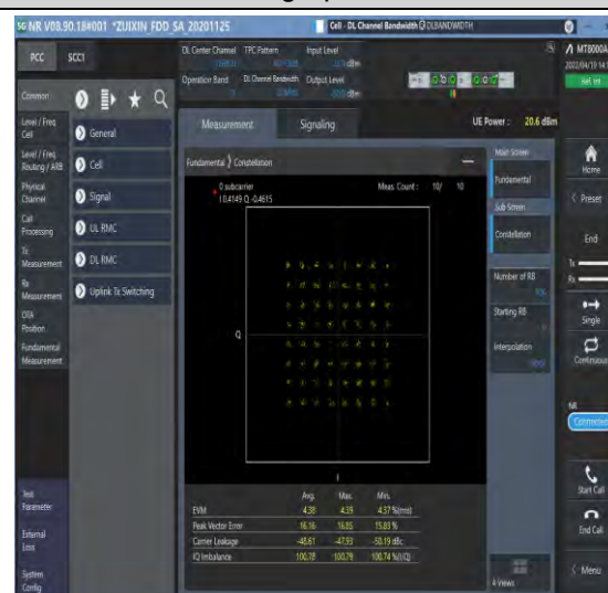
1-N71--15-20-M-8-CP-64QAM-Outer_Full-106@0-Ant1-see graph-PASS
