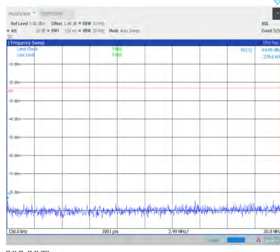
1-N71--15-20-M-1-DFT-PI2BPSK-Inner_1RB_Left-1 @1-0.15-30-Ant1--84.08--23-PASS
