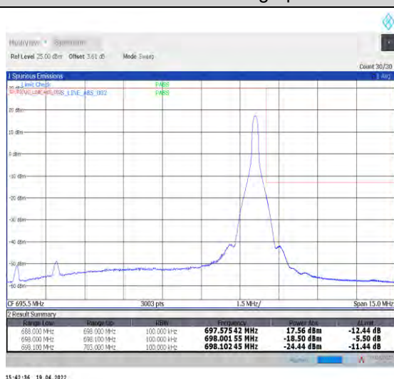
1-N71--15-10-H-5-CP-QPSK-Edge_1RB_Right-1@51-Ant1-PASS-see graph
