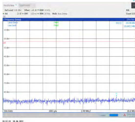
1-N71--15-20-H-1-DFT-PI2BPSK-Inner_1RB_Left-1 @1-0.15-30-Ant1--85.08--23-PASS
