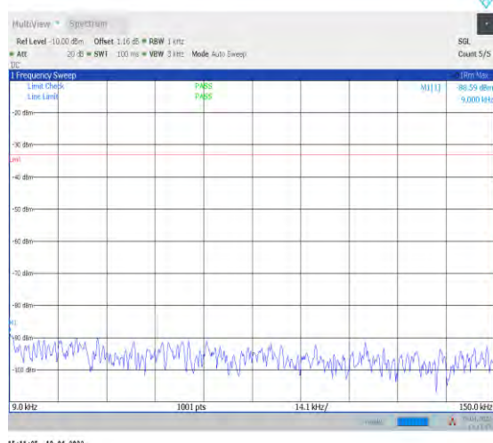
1-N71--15-20-M-1-DFT-PI2BPSK-Inner_1RB_Left-1 @1-0.009-0.15-Ant1--88.59--33-PASS
