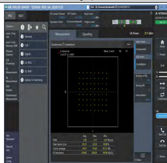
1-N71--15-20-M-4-DFT-64QAM-Outer_Full-100@0-A Ant1-see graph-PASS
