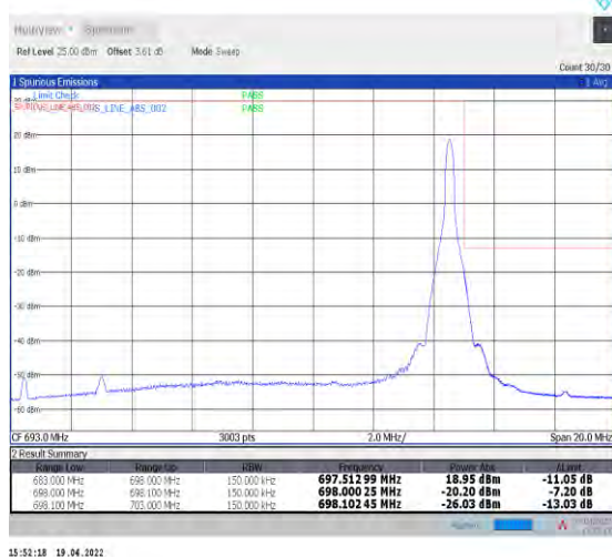
1-N71--15-15-H-5-CP-QPSK-Edge_1RB_Right-1@78-Ant1-PASS-see graph
