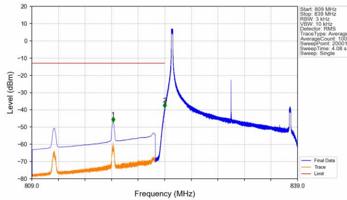
Band26b_15MHz_QPSK_LCH_831.5MHz_RB_1_0_NTNV
