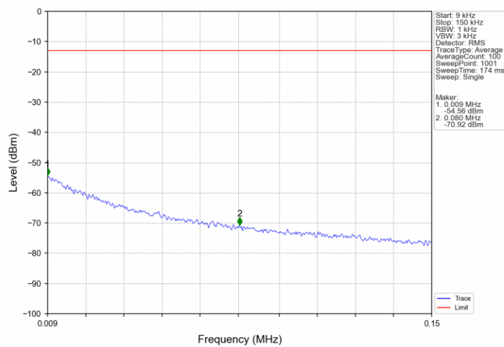
Band26b_15MHz_QPSK_LCH_831.5MHz_RB_1_0_NTNV
