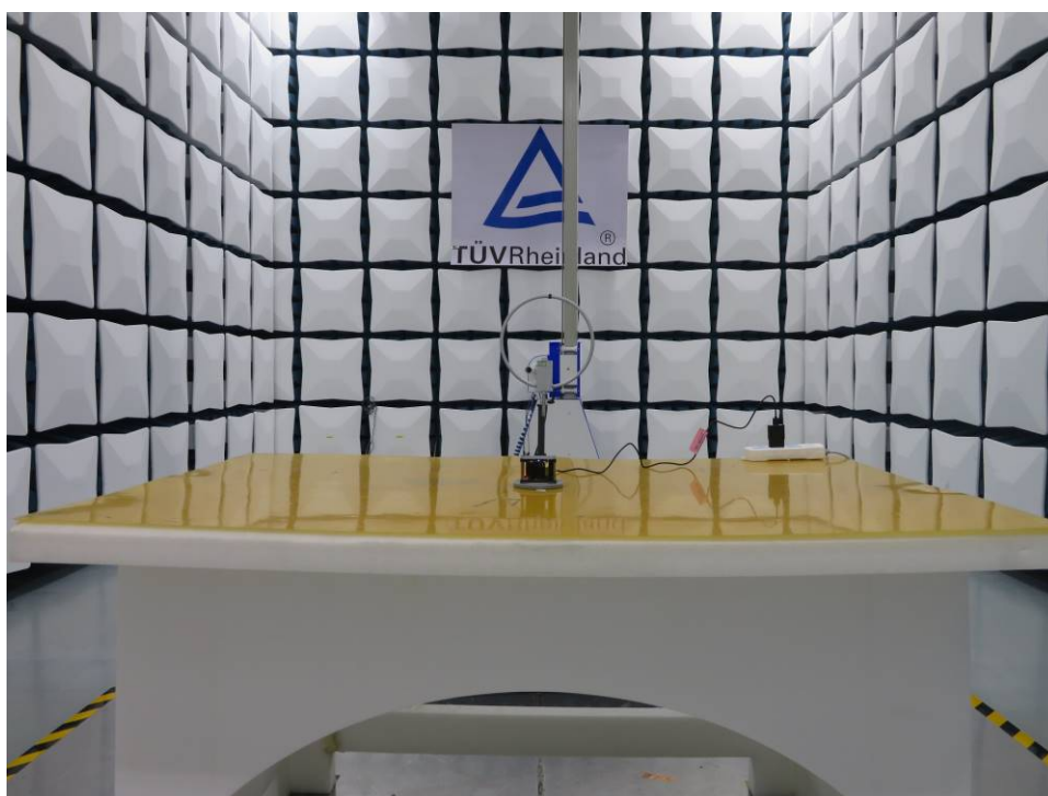
Photograph 1: Set-up photo for Radiated Emission, 9KHz - 30MHz
