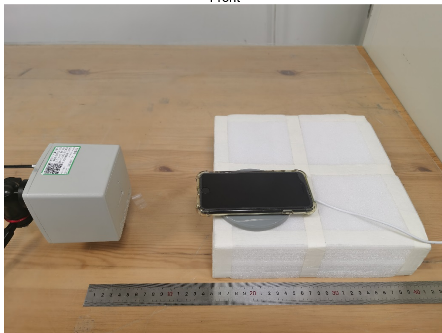
Photograph 4: Set-up photo for MPE Setup
