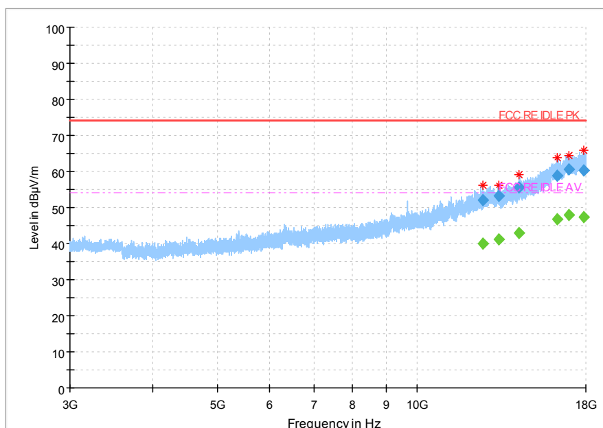
Fig.8.4 Radiated Spurious Emission (802.11 n-40MHz,Ch3,3GHz~18GHz)
