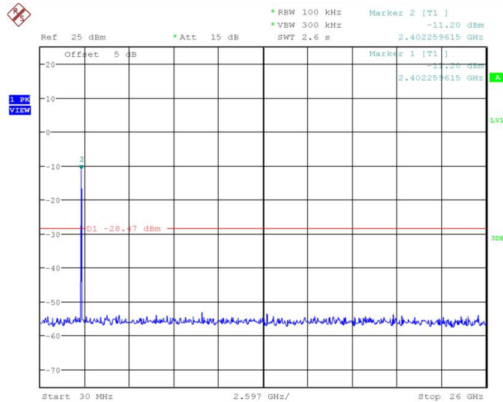
Fig.59 Conducted Spurious Emission (802.11n-40MHz, Ch3)
