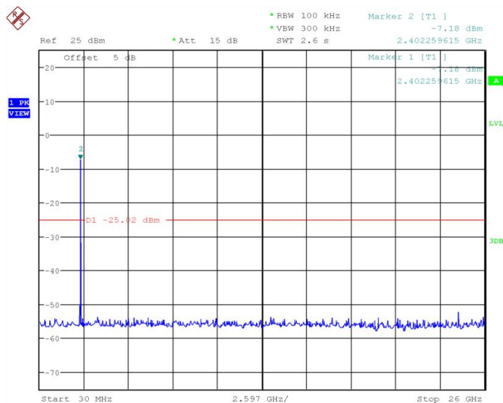
Fig.53 Conducted Spurious Emission (802.11n-20MHz, Ch1)
