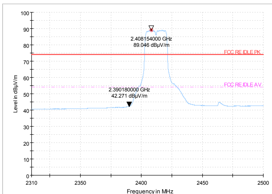
Fig.75 Radiated emission (Power): 802.11n, low channel
