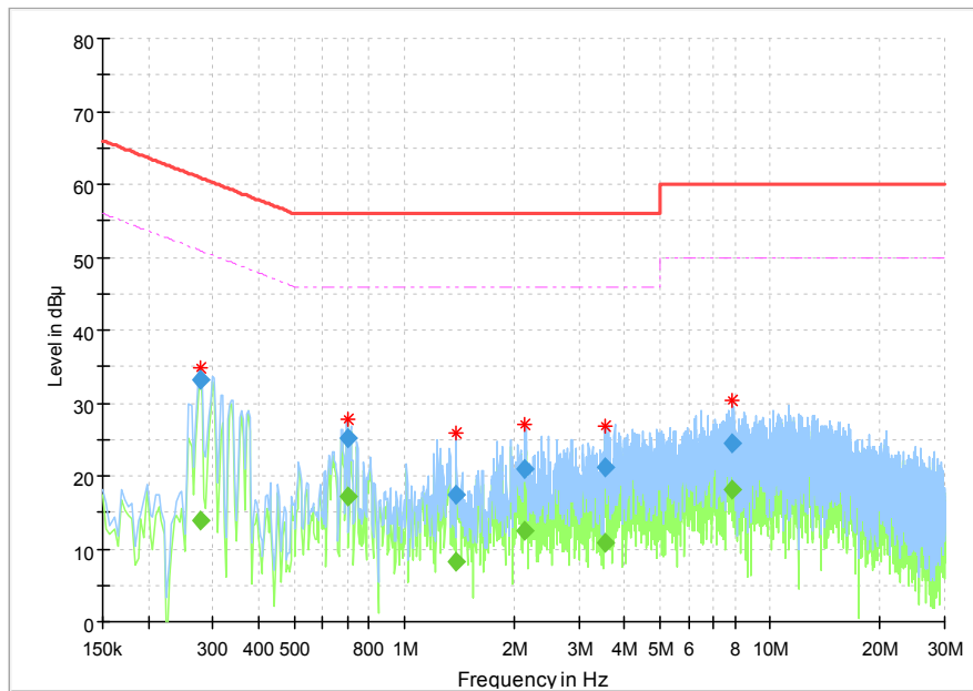
Fig.158 AC Powerline Conducted Emission
