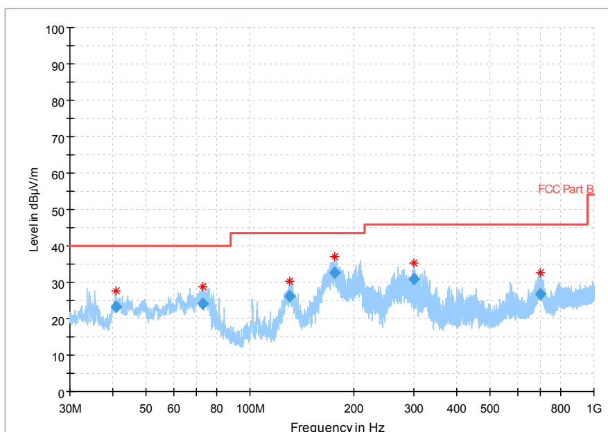
Fig.82 Radiated Spurious Emission (802.11 n-40MHz,Ch3,30MHz~1GHz)
