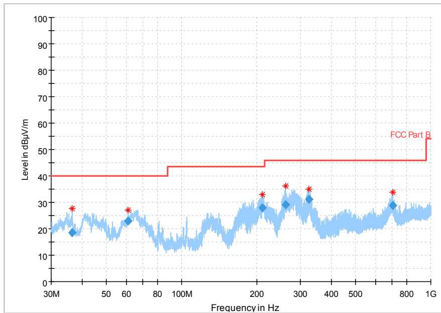
Fig.72 Radiated Spurious Emission (802.11g,Ch11,30MHz~1GHz)
