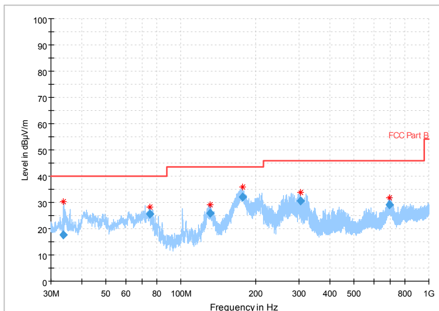
Fig.77 Radiated Spurious Emission (802.11 n-20MHz,Ch11,30MHz~1GHz)
