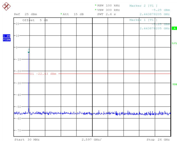
Fig.51 Conducted Spurious Emission (802.11g, Ch11)
