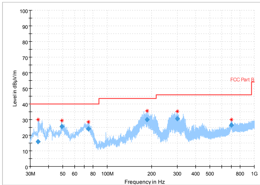
Fig.99 Radiated Spurious Emission (802.11b,Ch11,30MHz~1GHz)
