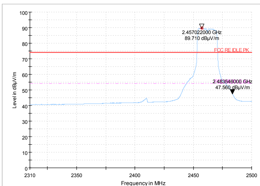
Fig.71 Radiated emission (Power): 802.11g, high channel
