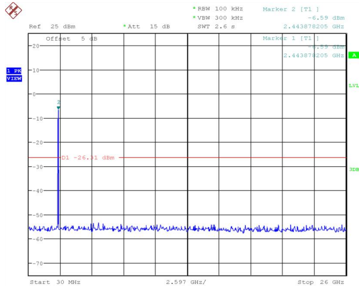
Fig.55 Conducted Spurious Emission (802.11n-20MHz, Ch6)
