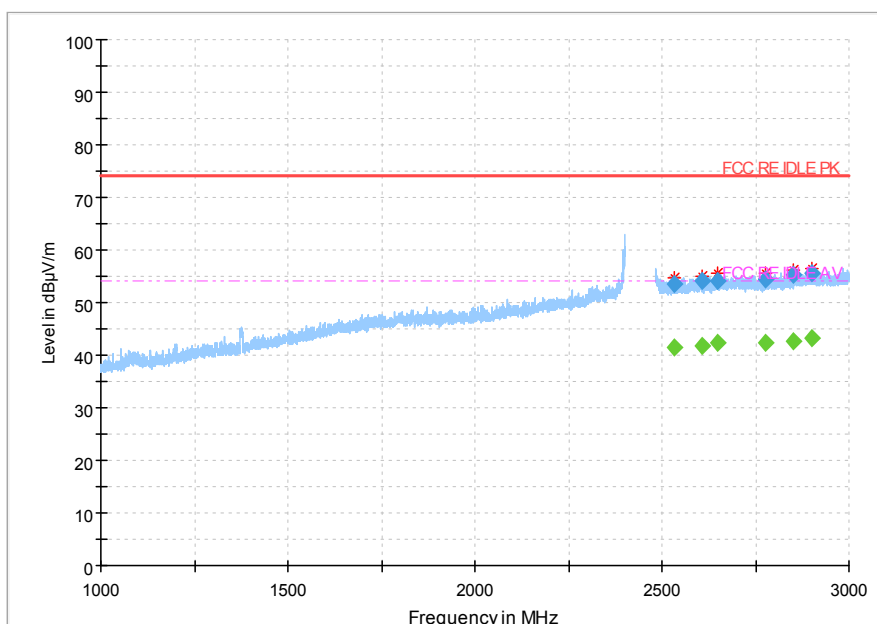
Fig.100 Radiated Spurious Emission (802.11b,Ch11,1GHz~3GHz)
