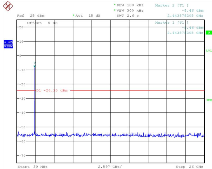
Fig.57 Conducted Spurious Emission (802.11n-20MHz, Ch11)
