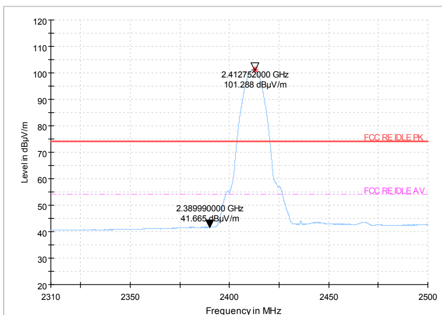
Fig.65 Radiated emission (Power): 802.11b, low channel
