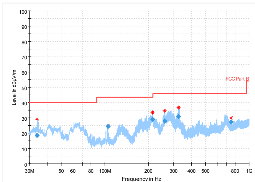
Fig.67 Radiated Spurious Emission (802.11b,Ch11,30MHz~1GHz)
