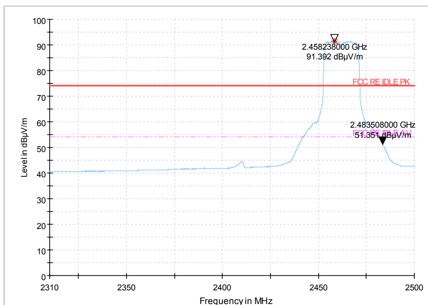
Fig.76 Radiated emission (Power): 802.11n, high channel
