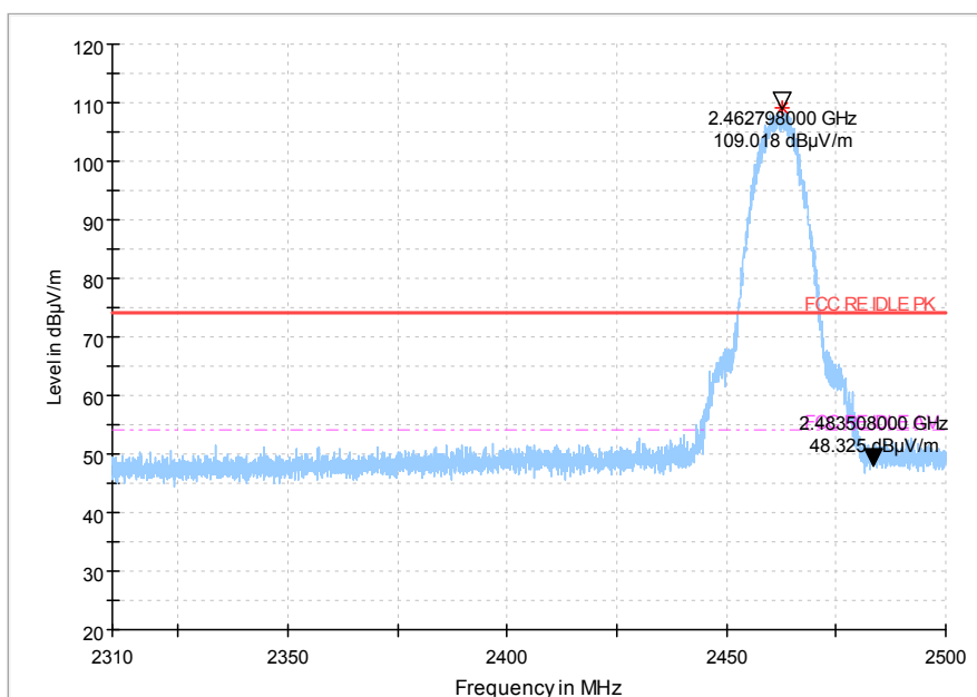
Fig.66 Radiated emission (Power): 802.11b, high channel
