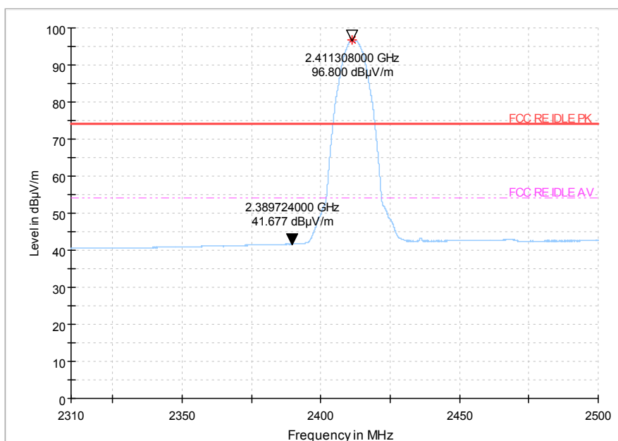
Fig.97 Radiated emission (Power): 802.11b, low channel
