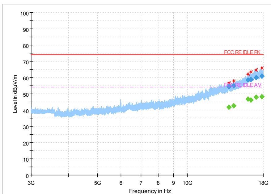
Fig.79 Radiated Spurious Emission (802.11 n-20MHz,Ch11,3GHz~18GHz)
