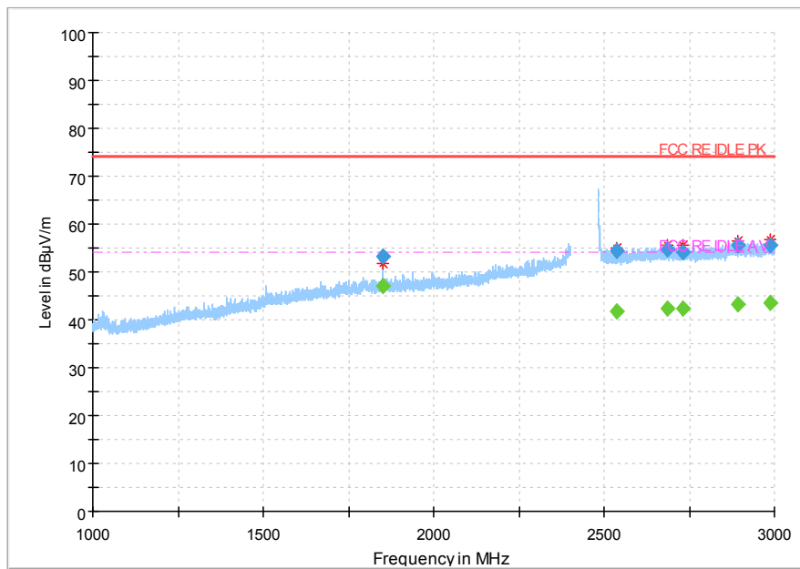
Fig.73 Radiated Spurious Emission (802.11g,Ch11,1GHz~3GHz)
