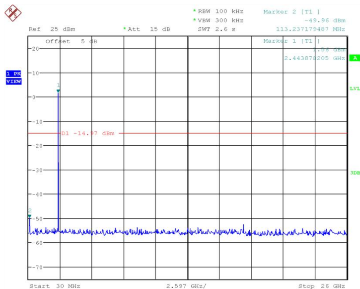
Fig.45 Conducted Spurious Emission (802.11b, Ch11)
