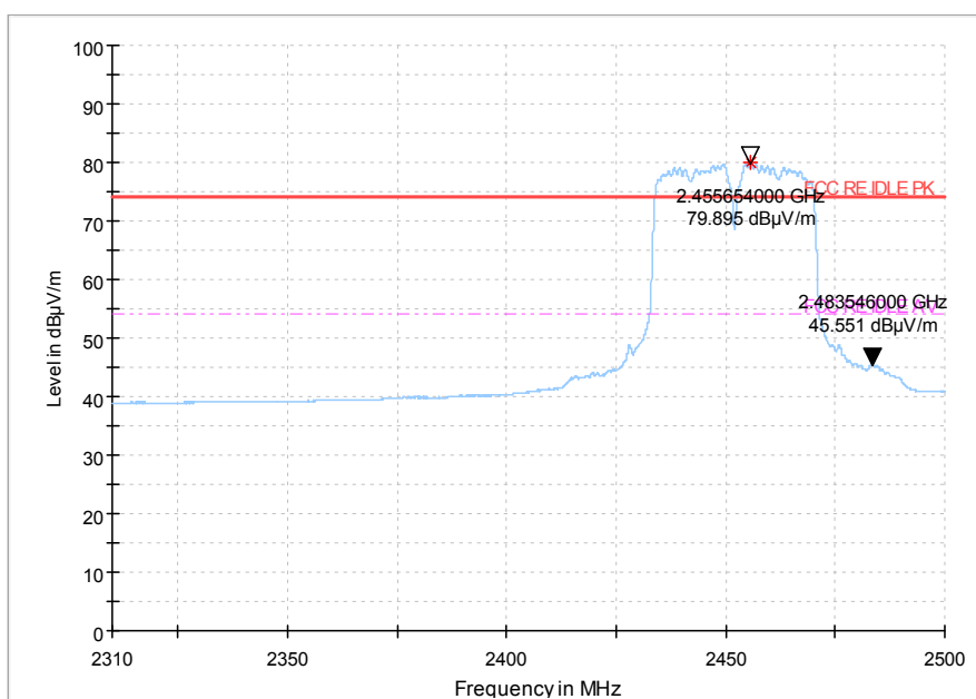
Fig.81 Radiated emission (Power): 802.11n (40M) , high channel
