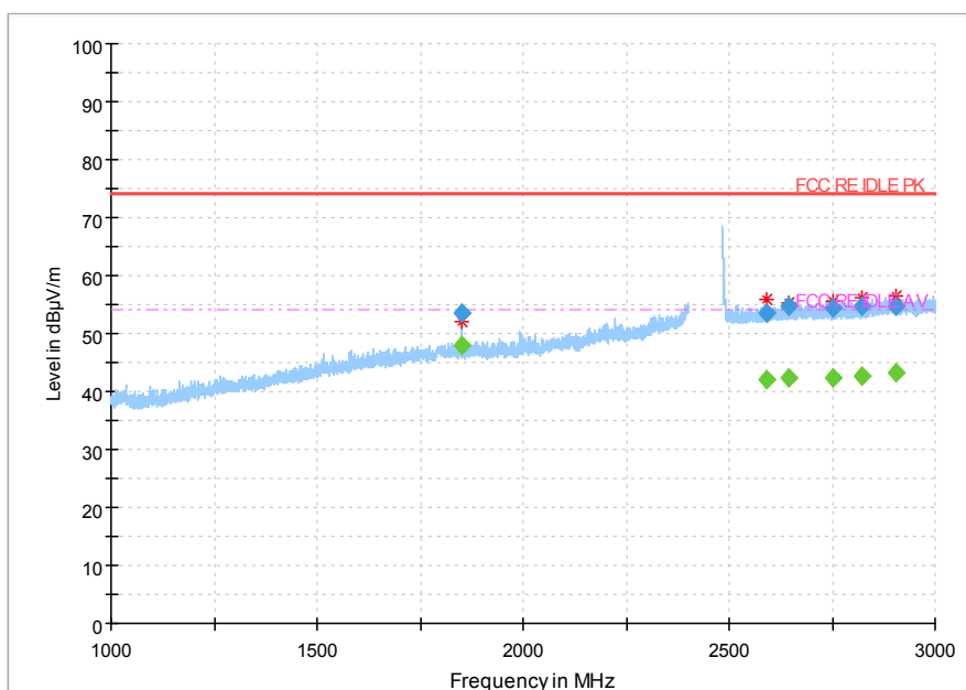
Fig.78 Radiated Spurious Emission (802.11 n-20MHz,Ch11,1GHz~3GHz)
