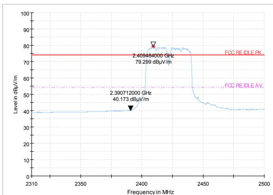
Fig.80 Radiated emission (Power): 802.11n (40M) , low channel
