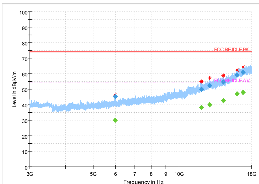
Fig.101 Radiated Spurious Emission (802.11b,Ch11,3GHz~18GHz)
