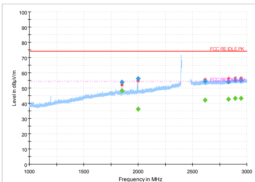
Fig.83 Radiated Spurious Emission (802.11 n-40MHz,Ch3,1GHz~3GHz)
