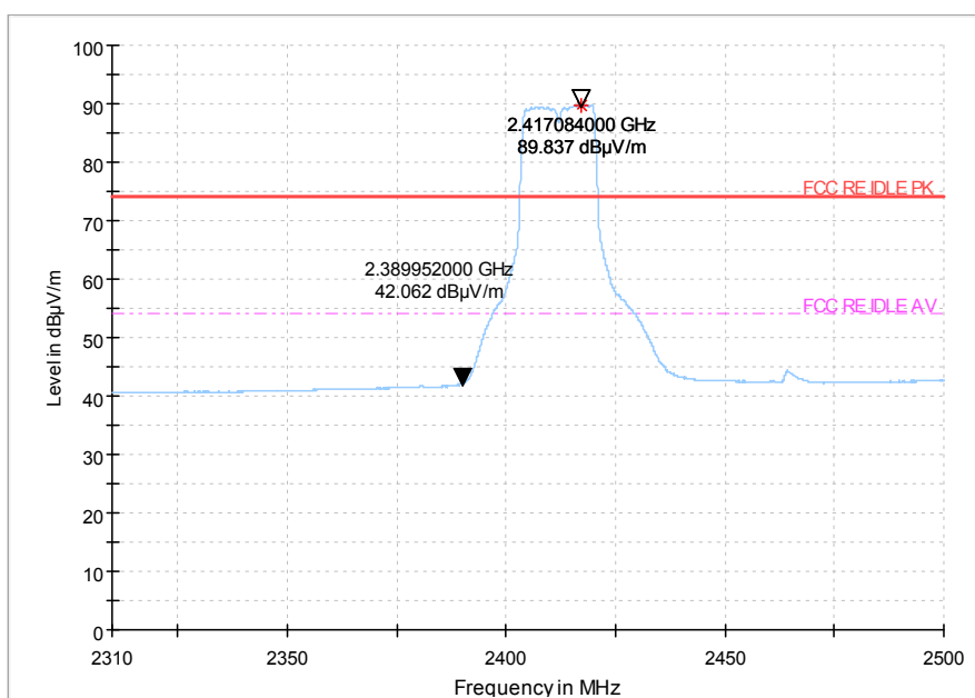
Fig.70 Radiated emission (Power): 802.11g, low channel
