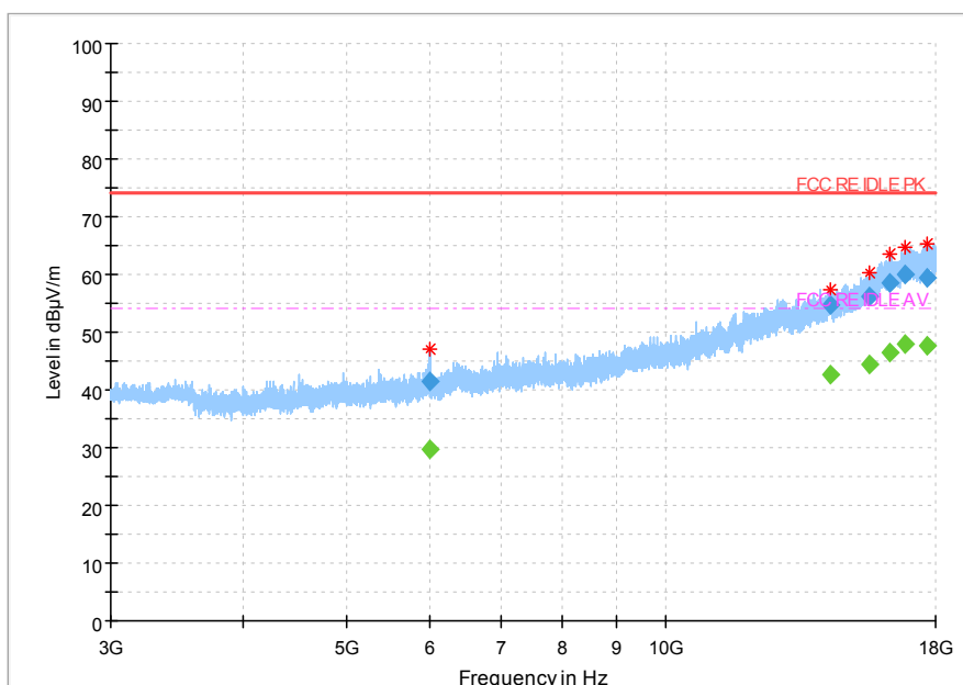
Fig.74 Radiated Spurious Emission (802.11g,Ch11,3GHz~18GHz)
