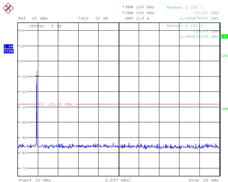
Fig.63 Conducted Spurious Emission (802.11n-40MHz, Ch9)
