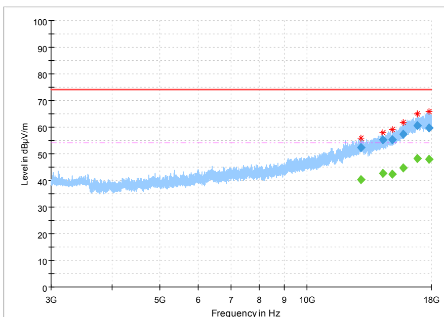
Fig.69 Radiated Spurious Emission (802.11b,Ch11,3GHz~18GHz)
