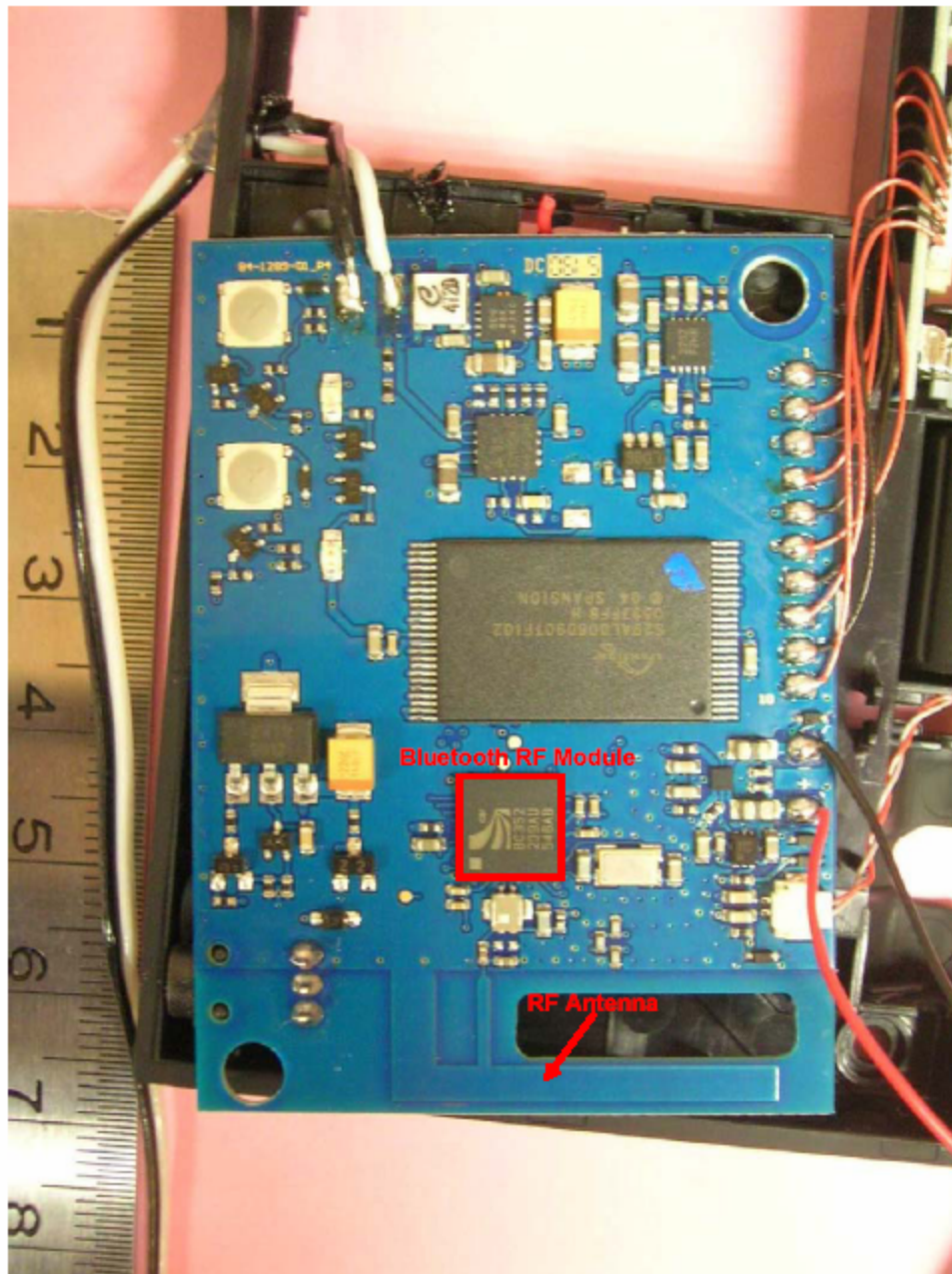
Main Unit - Component Side
