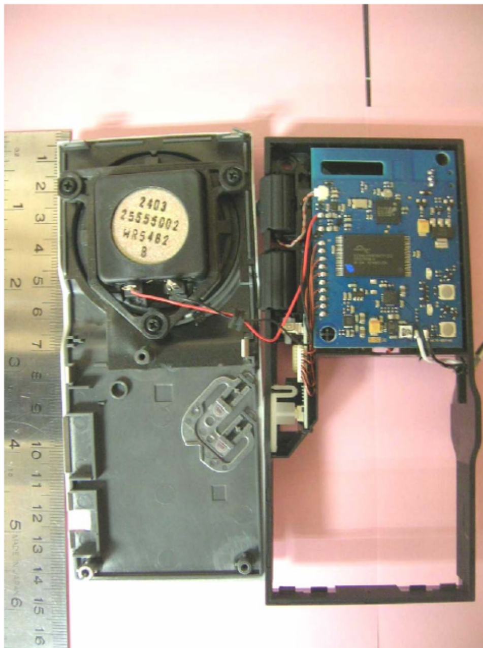
Main Unit - Internal View 2
