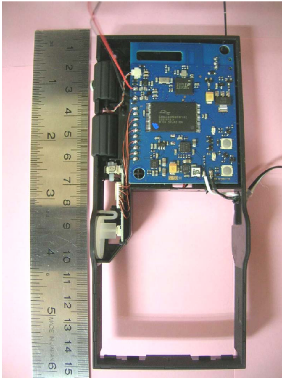
Main Unit - Internal View 4
