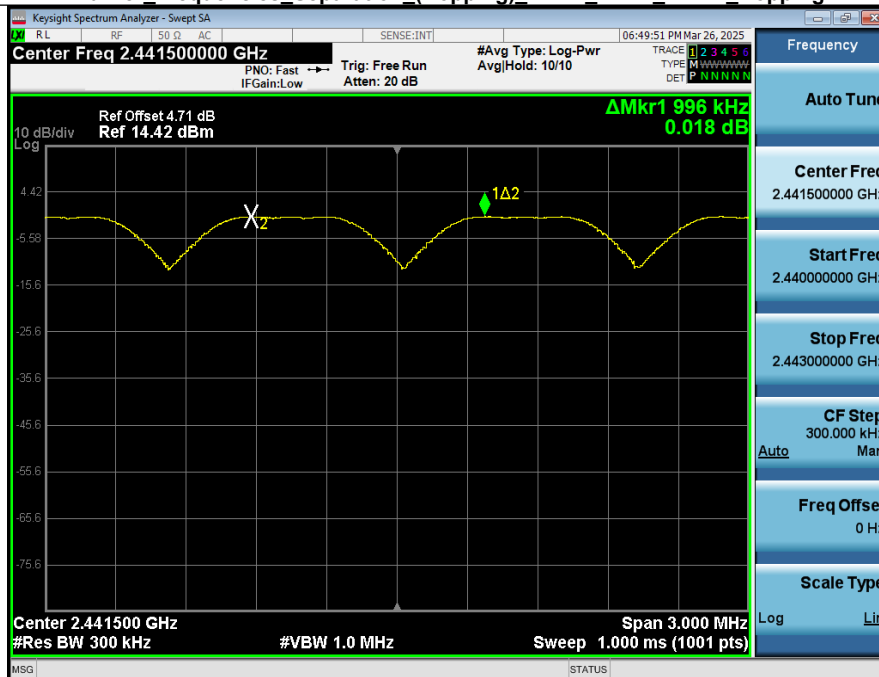
Carrier_Frequencies_Separation_(Hopping)_NVNT_ANT1_1-DH1_Hopping
