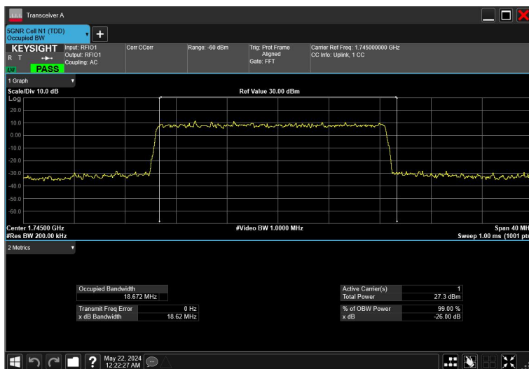
20MHz_15kHz_1745MHz_DFT-s-OFDM QPSK_RB100@0
