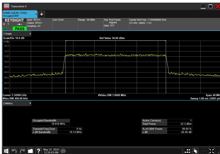
20MHz_15kHz_1745MHz_CP-OFDM 256 QAM_RB106@0
