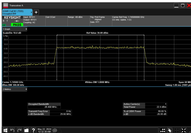
30MHz_15kHz_1745MHz_CP-OFDM 256 QAM_RB160@0
