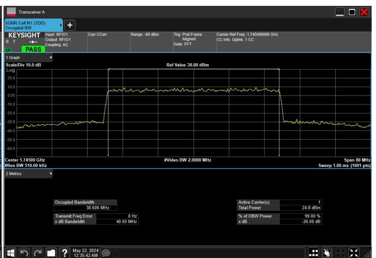
40MHz_15kHz_1745MHz_DFT-s-OFDM 256 QAM_RB216@0
