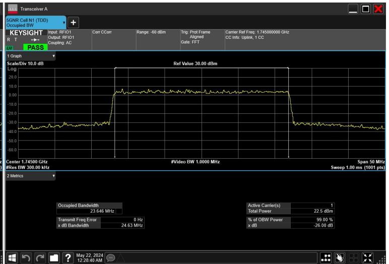
25MHz_15kHz_1745MHz_CP-OFDM 256 QAM_RB133@0
