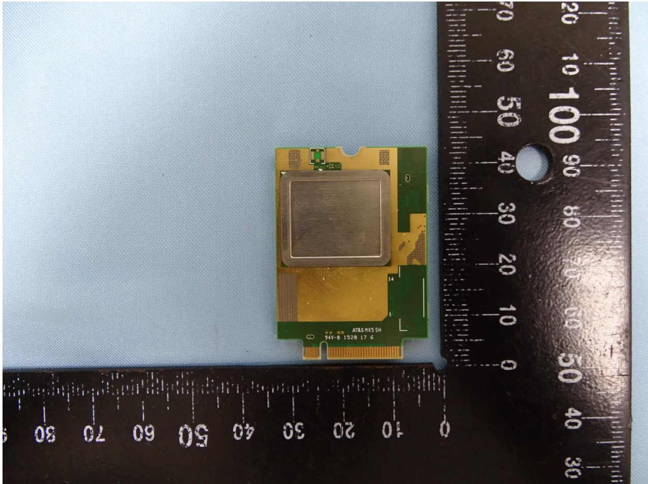
EUT: 5G WWAN Module (Brand Name: Foxconn / Model Name: T99W175)
