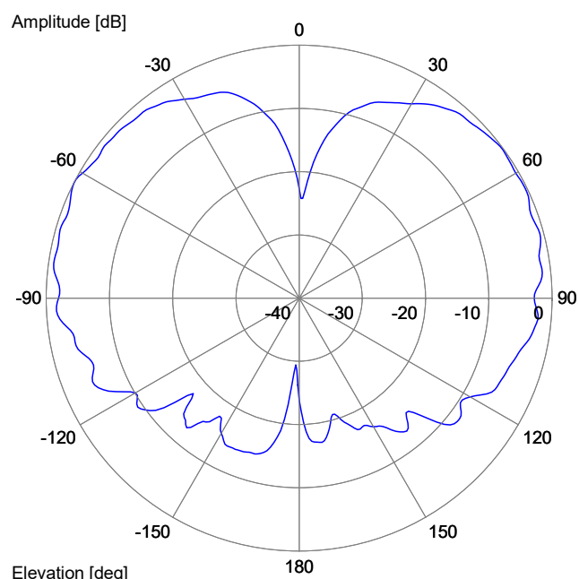
Radiation Pattern
