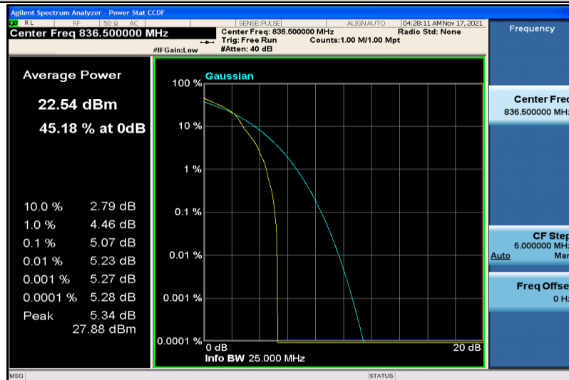
Band5-5MHz-16QAM-20525-1RB#0
