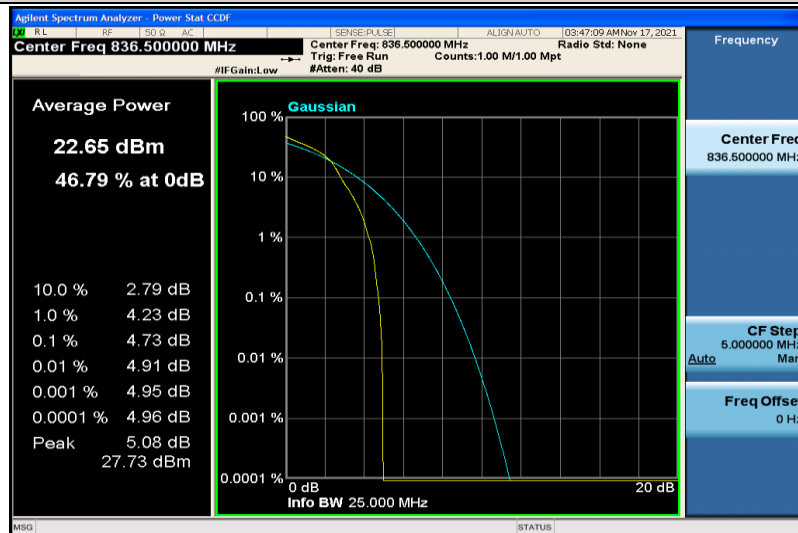
Band5-1.4MHz-16QAM-20525-1RB#0
