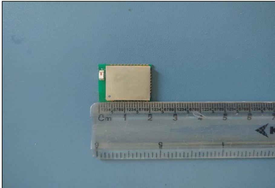
Photo 1: Dimensional View
