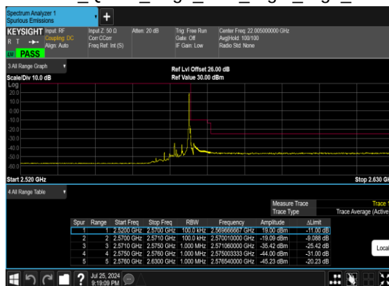
B66_N7(5M)_DFT-s- OFDM_QPSK_Edge_1RB_Right_High_CH
