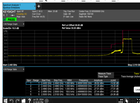
B66_N7(5M)_DFT-s- OFDM_QPSK_Outer_Full_Low_CH
