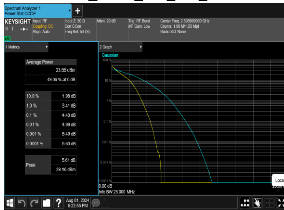
B4_N38(25M)_DFT-s-OFDM_PI_2- BPSK_Outer_Full_Mid_CH
