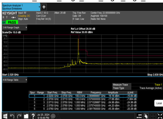
B66_N7(5M)_DFT-s- OFDM_BPSK_Edge_1RB_Right_High_CH
