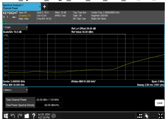
B66_N7(50M)_DFT-s- OFDM_QPSK_Edge_1RB_Left_Low_CH_CHP_PASS
