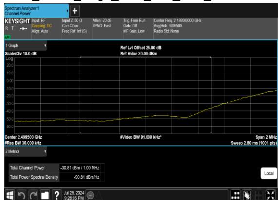
B66_N7(50M)_DFT-s- OFDM_BPSK_Edge_1RB_Left_Low_CH_CHP_PASS
