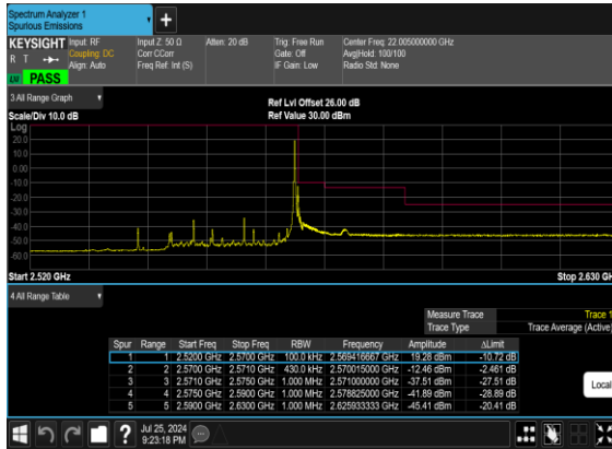
B66_N7(20M)_DFT-s- OFDM_BPSK_Edge_1RB_Right_High_CH
