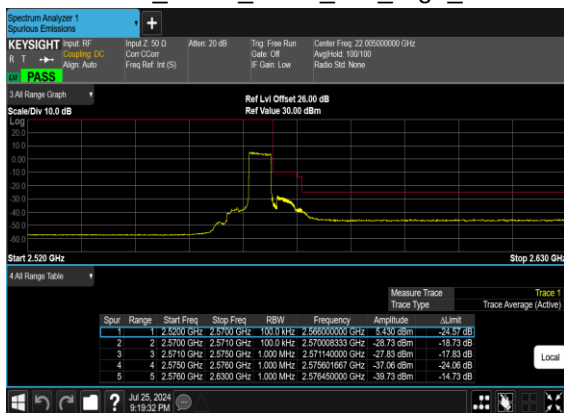
B66_N7(5M)_DFT-s- OFDM_BPSK_Outer_Full_High_CH
