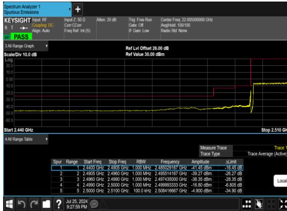
B66_N7(50M)_DFT-s- OFDM_BPSK_Outer_Full_Low_CH
