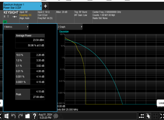
B4_N38(25M)_DFT-s-OFDM_PI_2- BPSK_Edge_1RB_Left_Mid_CH
