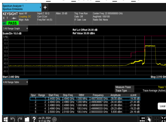
B66_N7(5M)_DFT-s- OFDM_BPSK_Outer_Full_Low_CH
