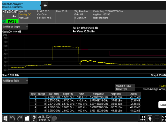
B66_N7(20M)_DFT-s- OFDM_BPSK_Outer_Full_High_CH
