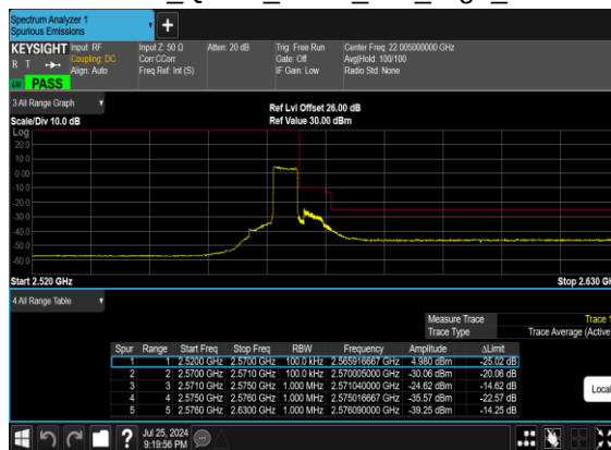
B66_N7(5M)_DFT-s- OFDM_QPSK_Outer_Full_High_CH
