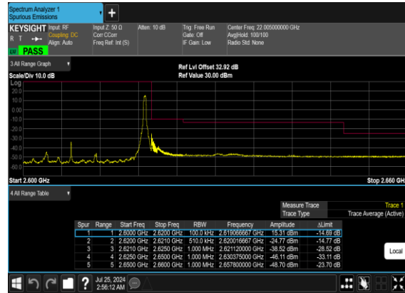
N38(25M)_DFT-s- OFDM_QPSK_Edge_1RB_Right_High_CH
