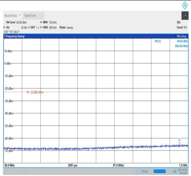
Band66_15MHz_QPSK_132597_1RB#74_30~1000_30~1000
