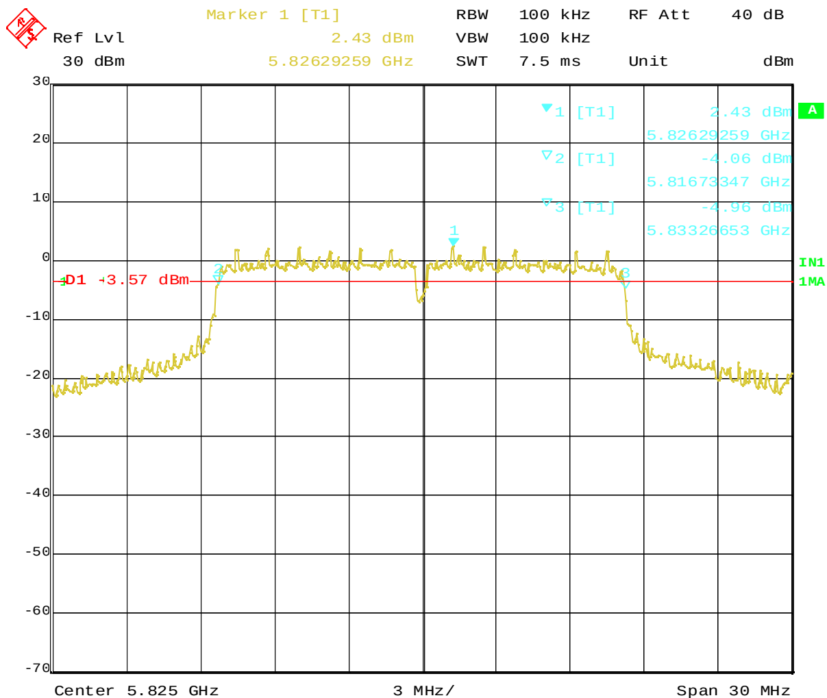
Plot 1-3. 6dB BW at 5825MHz (OFDM, 6Mbps)
