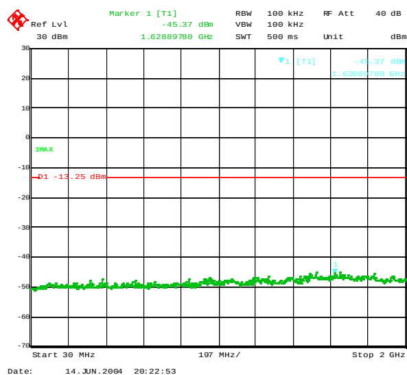
Plot 4-2. Out of band emissions around 2437MHz (DSSS, 11Mbps)
