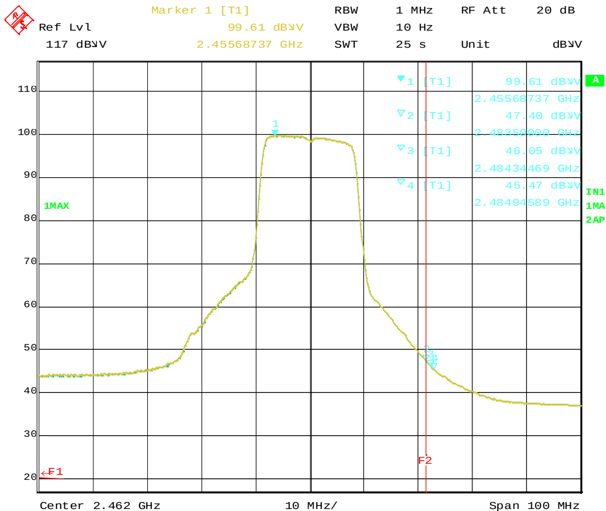
Plot 8-8 Ch.11 2462MHz TX, OFDM 6Mbps (Average), T40 Series
