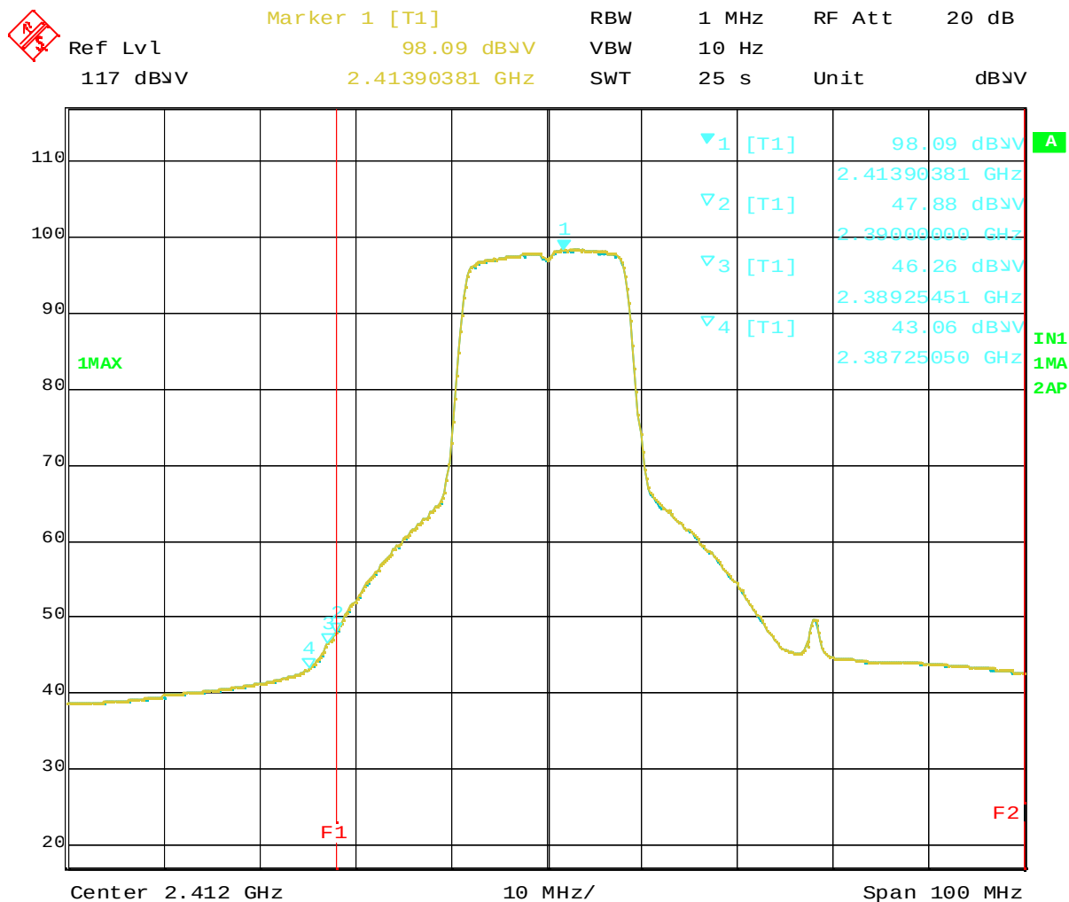
Plot 8-6 Ch.1 2412MHz TX, OFDM 6Mbps (Average), T40 Series
