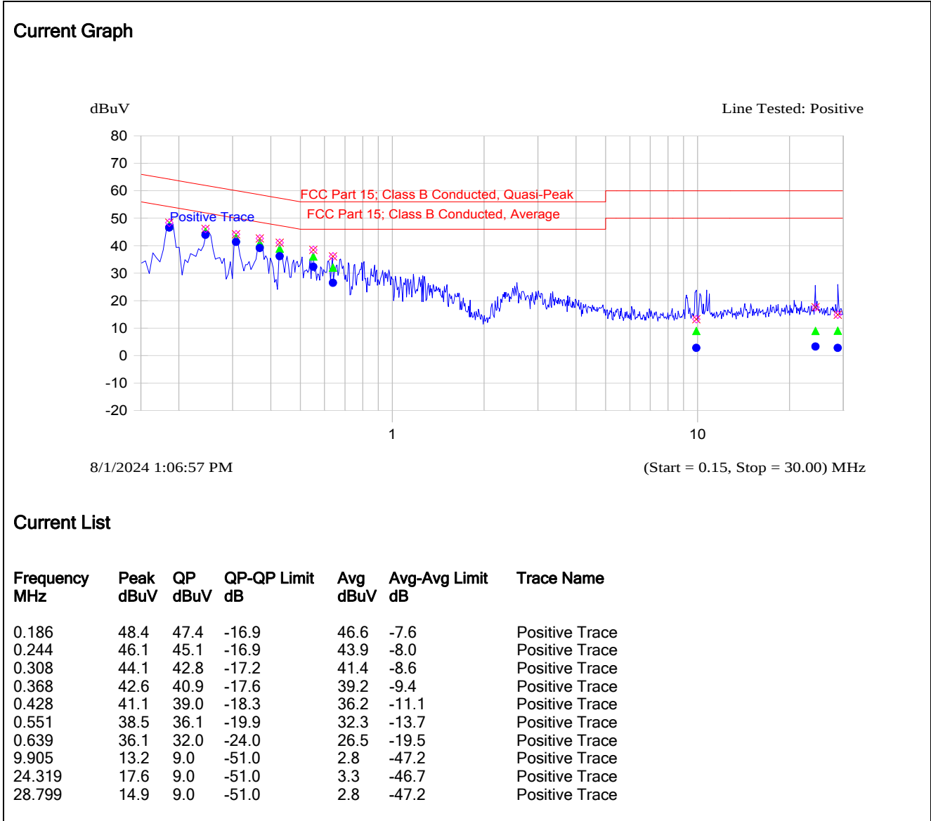
Plot 5.1.4.3. Power Line Conducted Emissions (BLE Rx Mode) Line Voltage: 3.6 VDC; Line Tested: Positive Trace
