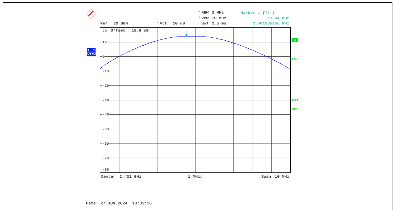
Plot 5.3.4.4. Maximum Peak Conducted Output Power, GFSK Modulation, Coded PHY, 125 kb/s, 2402 MHz
