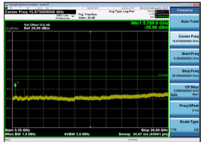
U-NII-1 ,Plot 3,5350MHz~26000MHz-802. 11ax(20MHz),5240MHz,Ant1
