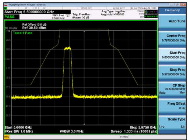
U-NII-3 ,Plot 1,Band Edge-802.11ax(20 MHz),5785MHz,Ant1
