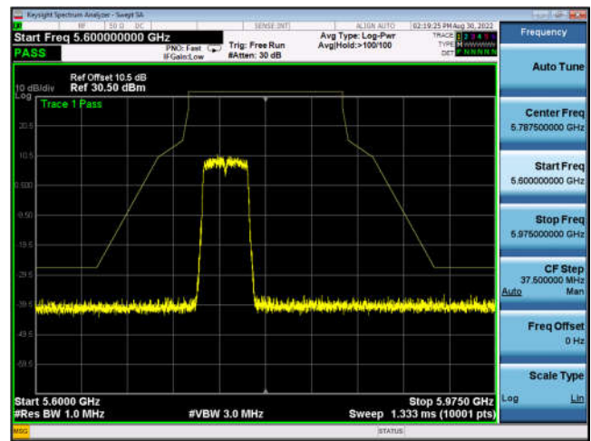
U-NII-3 ,Plot 1,Band Edge-802.11ax(40 MHz),5795MHz,Ant1
