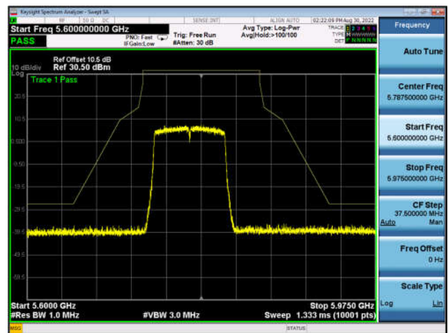
U-NII-3 ,Plot 1,Band Edge-802.11ac(80 MHz),5775MHz,Ant1
