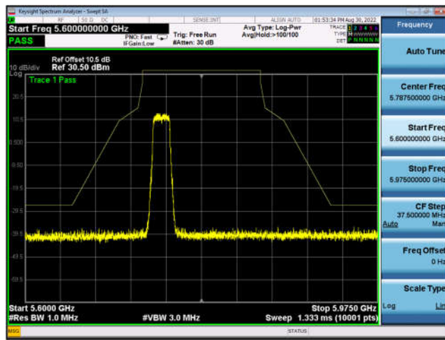
U-NII-3 ,Plot 1,Band Edge-802.11ax(20 MHz),5785MHz,Ant0
