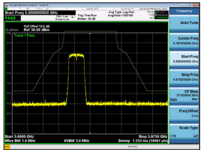
U-NII-3 ,Plot 1,Band Edge-802.11n(40M Hz),5795MHz,Ant1
