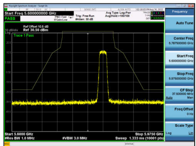
U-NII-3 ,Plot 1,Band Edge-802.11ax(20 MHz),5825MHz,Ant1
