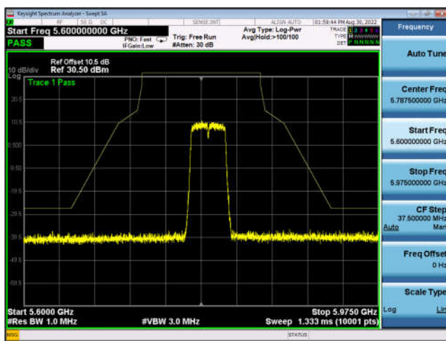
U-NII-3 ,Plot 1,Band Edge-802.11ax(80 MHz),5775MHz,Ant0
