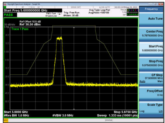
U-NII-3 ,Plot 1,Band Edge-802.11a(20 Hz),5785MHz,Ant1
