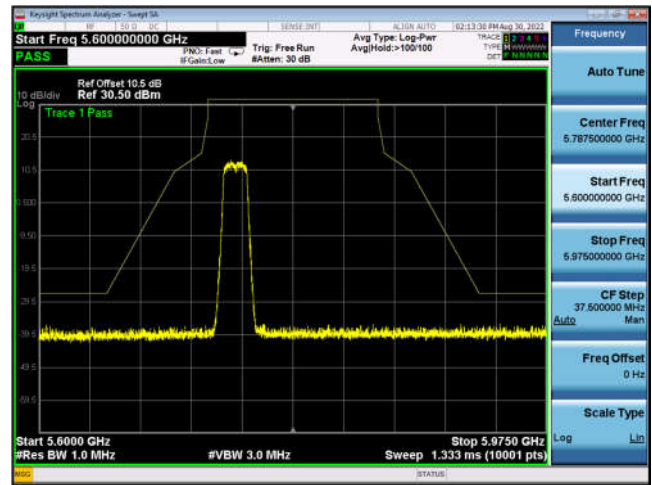
U-NII-3 ,Plot 1,Band Edge-802.11ac(20 MHz),5785MHz,Ant1
