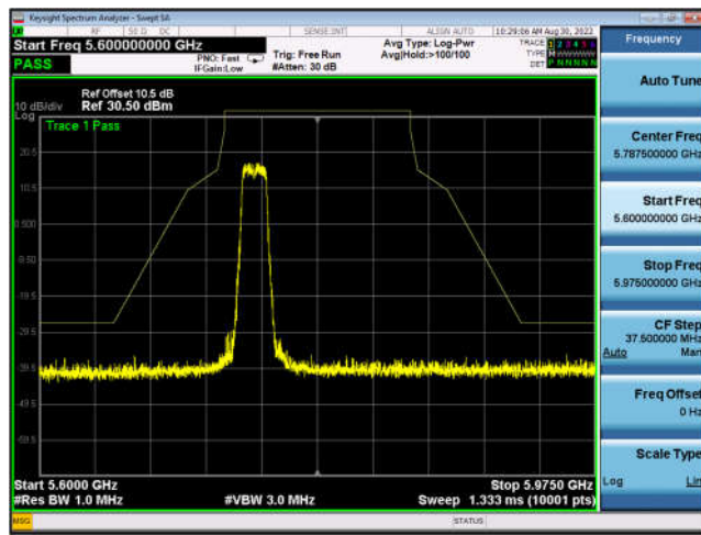
U-NII-3 ,Plot 1,Band Edge-802.11a(20 Hz),5785MHz,Ant0
