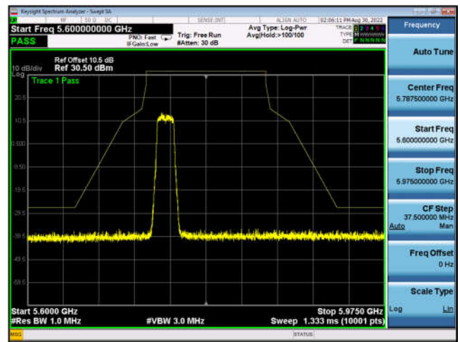
U-NII-3 ,Plot 1,Band Edge-802.11n(20 Hz),5785MHz,Ant1
