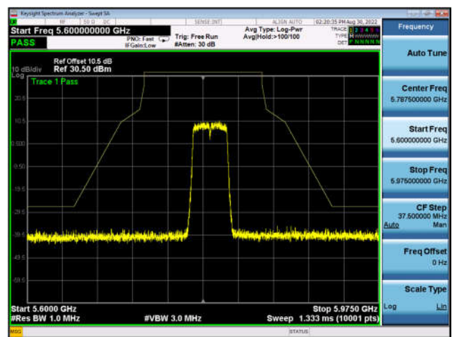
U-NII-3 ,Plot 1,Band Edge-802.11ax(80 MHz),5775MHz,Ant1
