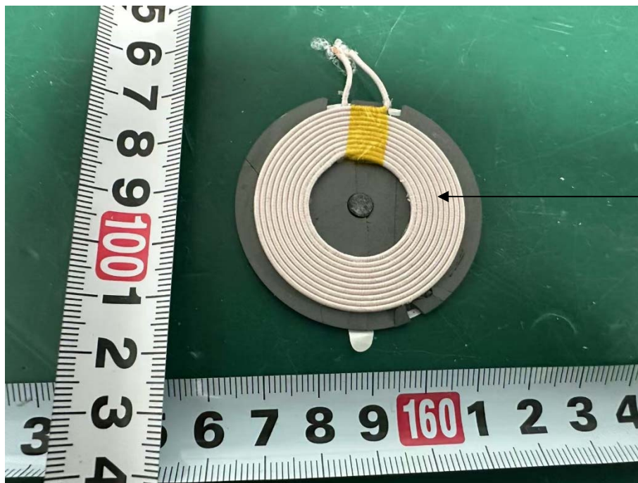
Coil Antenna
