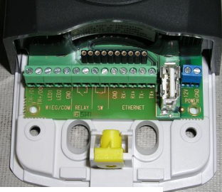
MA110 I-O connections
