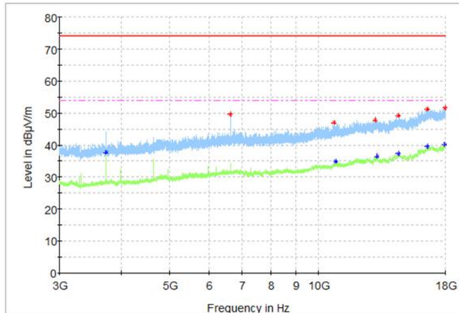
Fig.26 Radiated Spurious Emission (Ch39, 3 GHz - 18 GHz), 1M
