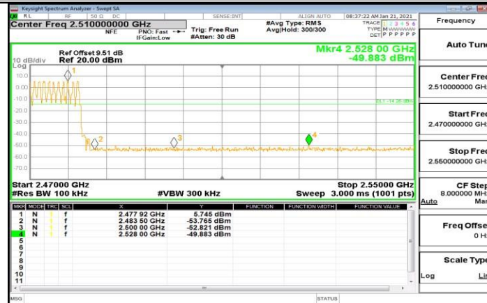
DH5_Ant1_High_Hop_2480
