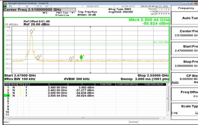
3DH5_Ant1_High_2480
