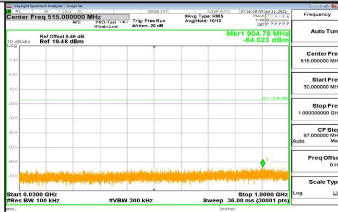
3DH5_Ant1_2402_30~1000
