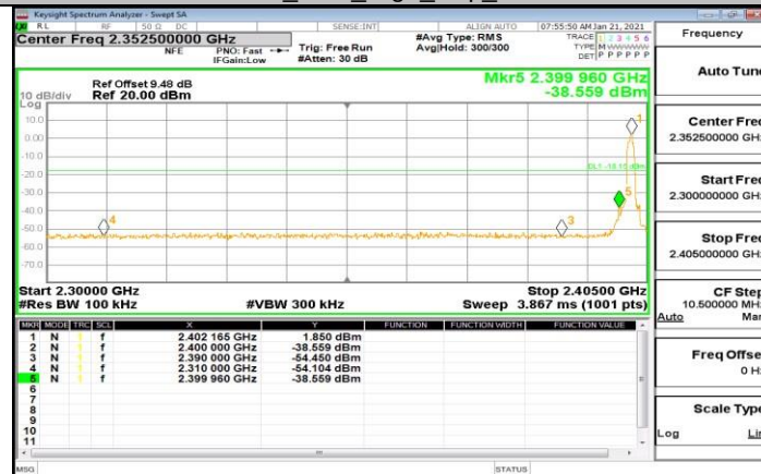
3DH5_Ant1_Low_2402
