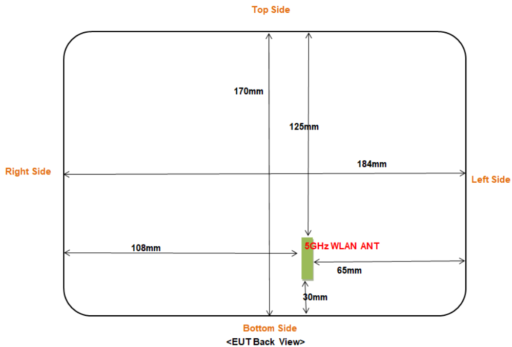
Fig 7.1 Block Diagram for EUT Antenna Position EUT Size: Long*Width*Height=184mm*170mm*60mm
