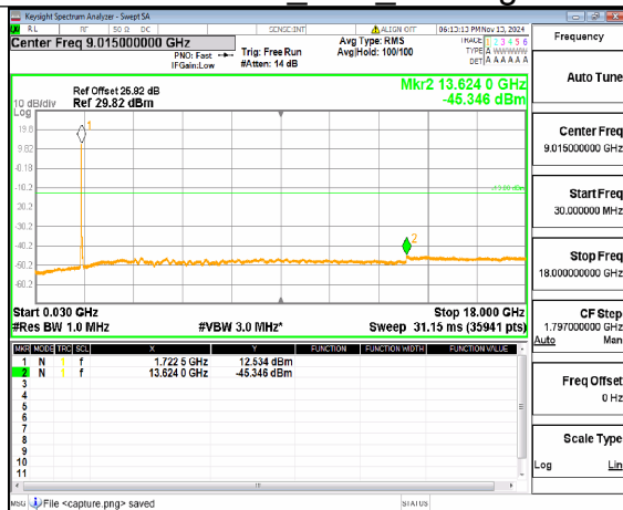
n66 (30MHz-18GHz) 15M DFT-s-OFDM QPSK Outer Full Low
