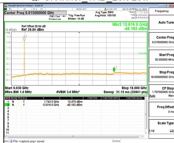
n66 (30MHz-18GHz) 15M DFT-s-OFDM QPSK Outer Full Mid
