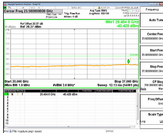
n41 (20GHz-27GHz) 50M DFT-s-OFDM QPSK Outer_Full High
